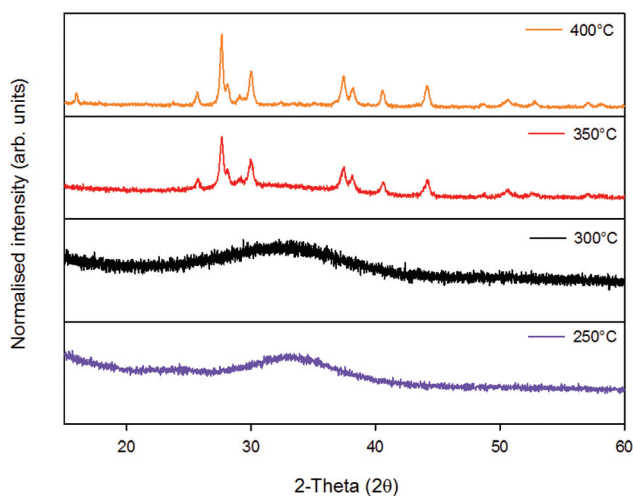
Fig. 2 XRD data for the precipitate of \text{NaV}(\text{SO}_4)_2 in the range of 250–400 °C (0.5 °C \text{min}^{-1} /12 hours) under Nitrogen (Co \text{K}\alpha_1/\text{K}\alpha_2 ).
