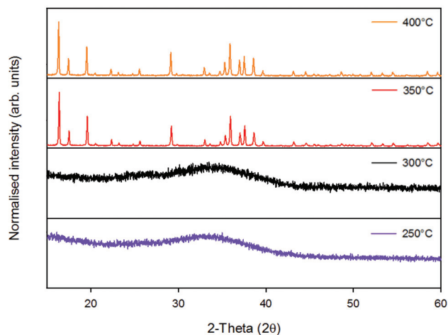
Fig. 3 XRD data for the precipitate of \text{Na}_2\text{VO}(\text{SO}_4)_2 in the range of 250–400 °C (0.5 °C \text{min}^{-1} /4 hours) in air (Co \text{K}\alpha_1/\text{K}\alpha_2 ).
