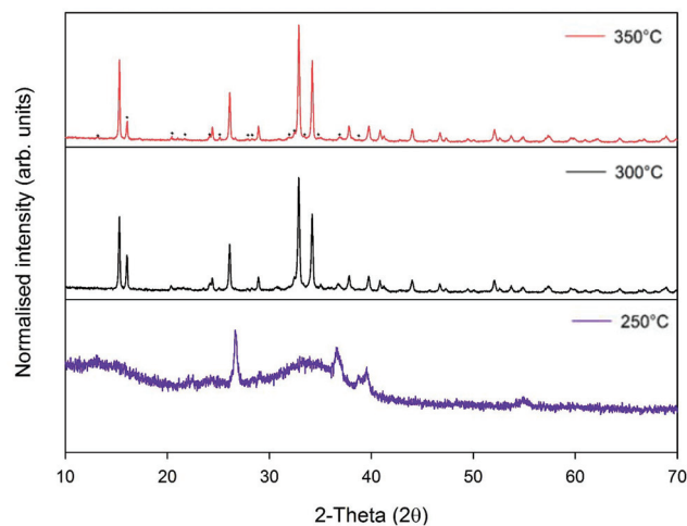
Fig. 4 XRD data for the precipitate of \text{Na}_3\text{V}(\text{SO}_4)_3 in the range of 250–350 °C (0.5 °C \text{min}^{-1} /12 hours) under Nitrogen. Impurity peaks (in the 350 °C composition) have been labelled with black diamonds (◆) (Co \text{K}\alpha_1/\text{K}\alpha_2 ).
