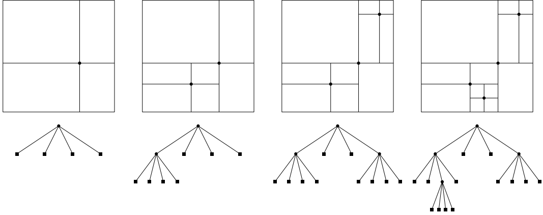
Figure 1: The first four steps in the quadtree construction of the partition, and of the corresponding trees. The placeholders are marked with squares while the actual nodes, which ‘store’ one of the points, are depicted with disks.
