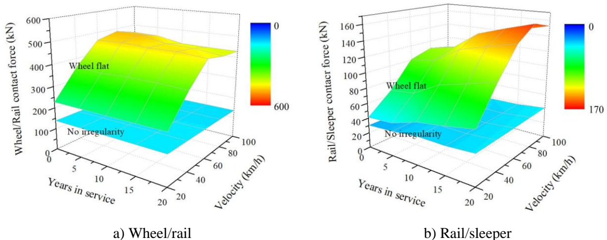
Figure 4. Contact force contour at different velocities over time.
