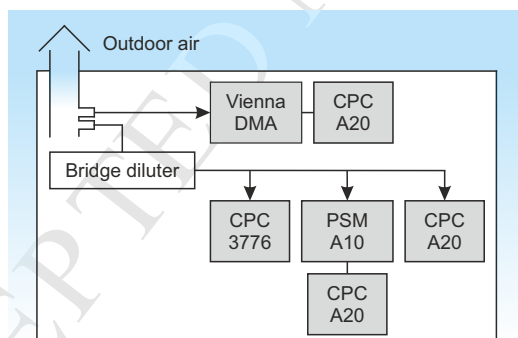
Figure 1: The measurement setup. The outdoor air sample was drawn from the roof into the measurement station, diluted with a bridge diluter and conducted to the condensation particle counters (CPCs) and particle size magnifier (PSM). The differential mobility particle sizer (DMPS) was connected to a separate sampling line before the bridge diluter.
