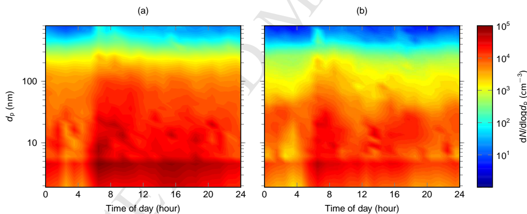
Figure 8: Diurnal variation of particle size distributions on weekdays with wind blowing from the road (a) and from the background direction (b).
