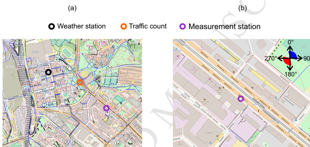
Figure 3: Maps of the measurement locations. (a) Locations of the traffic count, the Pasila weather station and the measurement station, (b) the surroundings of the measurement station and the wind direction sectors used throughout this study on the map. © OpenStreetMap contributors.
