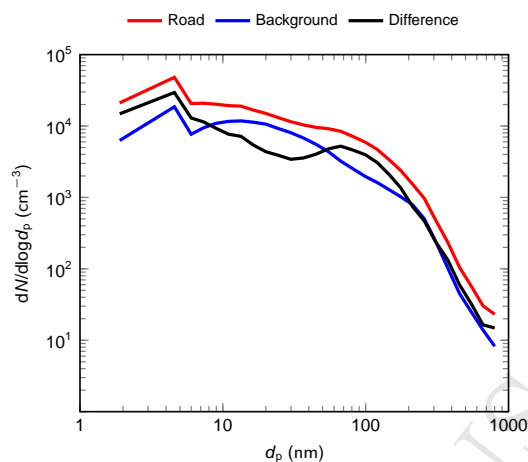
Figure 7: Average particle size distributions from two wind direction sectors, road and background, and the difference of these wind sector distributions. Distributions consist of differential mobility particle sizer (DMPS) distributions from 6 to 800 nm and two smaller size classes calculated from the data of the particle size magnifier (PSM) and condensation particle counters (CPCs).
