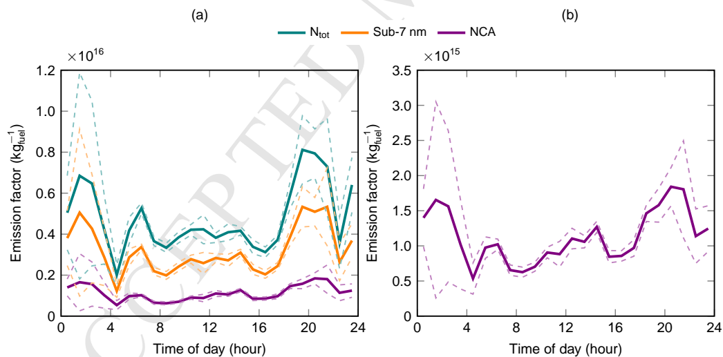
Figure 10: (a) Diurnal variation of emission factors of nanocluster aerosol (NCA), sub-7 nm particles and all particles. (b) Diurnal variation of NCA emission factors presented more closely. Dashed lines in both figures present the 95 % confidence bounds.
