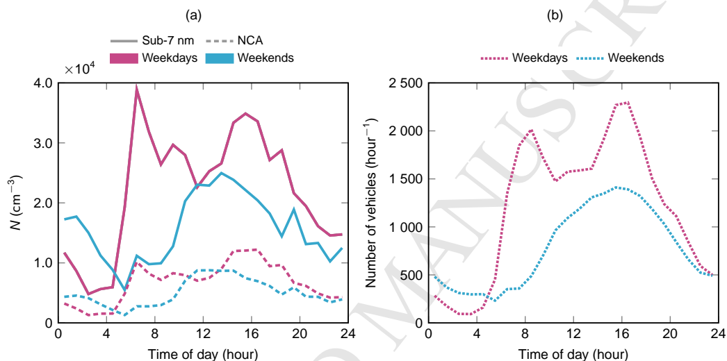
Figure 4: (a) Average diurnal variations of the nanocluster aerosol (NCA, dashed line) and sub-7 nm particle (solid line) concentrations separately for weekdays and weekends. (b) Average diurnal variation of traffic (vehicles \text{hour}^{-1} ) along the street Mäkelänkatu during the measurement campaign. The traffic count point was located in an intersection near the measurement station. Traffic data from the City of Helsinki.
