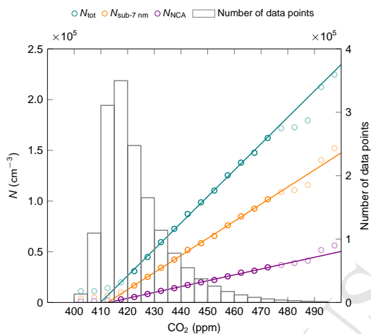
Figure 9: Total particle number concentration and the concentrations of sub-7 nm particles and nanocluster aerosol (NCA) as a function of simultaneously measured \text{CO}_2 concentration. Data points are averages of number concentrations in 5 ppm \text{CO}_2 intervals. Number of averaged data points in each \text{CO}_2 interval is presented as a histogram. Points averaged from less than 5000 data points and those considered as background were excluded from linear fits and plotted with lighter colors.
