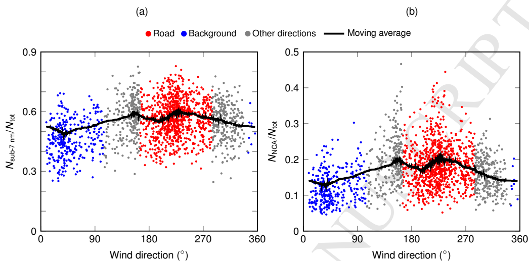
Figure 6: The concentrations of (a) sub-7 nm particles and (b) nanocluster aerosol (NCA) relative to total particle number concentration as a function of wind direction. Each data point is an average over 15 minutes and black line presents the moving average with respect to wind direction. Data periods with low traffic flow have been excluded. Wind directions classified as coming from the road are colored with red, background directions with blue and other directions with gray. Note the different scales of the y-axes.
