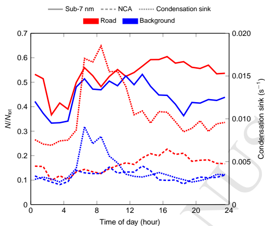
Figure 5: Relative diurnal variations of the nanocluster aerosol (NCA) and sub-7 nm particle concentrations in two wind direction sectors on weekdays. Red color presents wind blowing from the road to the measurement station, blue from the opposite background direction. For comparison, diurnal variation of the condensation sink calculated from differential mobility particle sizer (DMPS) distributions is also included.
