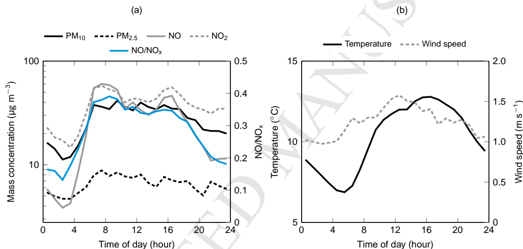
Figure 2: (a) Diurnal variations of NO, NO 2 , PM 10 , PM 2.5 and the NO/NO x ratio on weekdays during the measurement campaign. Note the logarithmic scale of the left y-axis. (b) Diurnal variation of temperature and wind speed during the measurement campaign.
