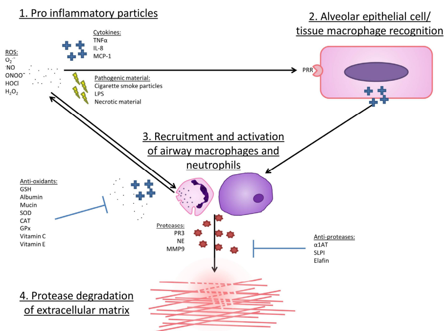
Figure 2. Process of tissue damage in chronic obstructive pulmonary disease (COPD). 1. Influx of pro-inflammatory particles into lung. 2. Particles bind PRRs on the surface of lung epithelial or tissue macrophages, instigating a signalling cascade culminating in the release of pro-inflammatory cytokines. 3. Cytokines encourage the recruitment, migration and activation of peripheral neutrophils and monocytes, the latter of which mature to alveolar macrophages once recruited. Activation of these cells results in the further cytokine release, proteases and ROS, in turn fueling further recruitment and activation. In health, anti-proteases and anti-oxidants are present in very high levels, preventing excess damage to surrounding tissues, and limiting a positive feedback loop. In COPD, these levels may be lacking, resulting in increased areas of obligate tissue damage. 4. If insufficiently inhibited, proteases will degrade extracellular matrix, leading to tissue destruction and pathologies seen in COPD. O_2^{\cdot -} , superoxide anion; \cdot NO , nitric oxide; SOD, superoxide dismutase; H_2O_2 , hydrogen peroxide; CAT, catalase; GPx, glutathione peroxidase; MPO, myeloperoxidase; HOCl , hypochlorous acid; ONOO^{\cdot -} , peroxynitrite; TNF \alpha , tumour necrosis factor \alpha ; IL8, Interleukin 8; MCP-1, monocyte chemoattractant protein 1; LPS, lipopolysaccharide; PRR, pattern recognition receptor; GSH, glutathione; PR3, proteinase 3; NE, neutrophil elastase; MMP9, matrix metalloproteinase 9; \alpha 1AT , \alpha 1 antitrypsin; SLPI, secretory leukocyte protease inhibitor.
