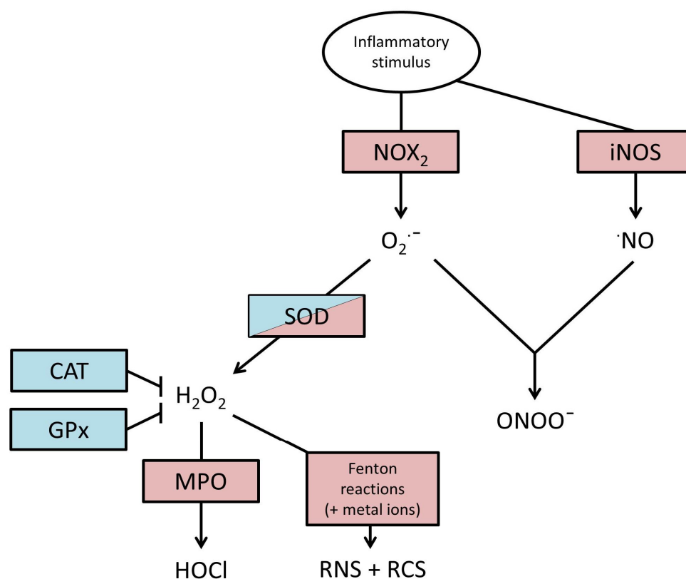
Figure 1. Molecular production of reactive species. Initiated by an inflammatory stimulus, a cascade begins that results in a variety of oxidative agents. Red boxes represent pro-inflammatory enzymes, whilst blue boxes represent anti-inflammatory enzymes. Superoxide dismutase (SOD) may be classed as both as its substrate and product are both capable of causing harm. NOX2, nicotinamide adenine dinucleotide phosphate(NADPH)-oxidase; iNOS, inducible nitric oxide synthase; \text{O}_2\cdot^- , superoxide anion; \cdot\text{NO} , nitric oxide; SOD, superoxide dismutase; \text{H}_2\text{O}_2 , hydrogen peroxide; CAT, catalase; GPx, glutathione peroxidase; MPO, myeloperoxidase; \text{HOCl} , hypochlorous acid; RCS + RNS, reactive nitrogen species + reactive carbon species; \text{ONOO}^- , peroxynitrite.
