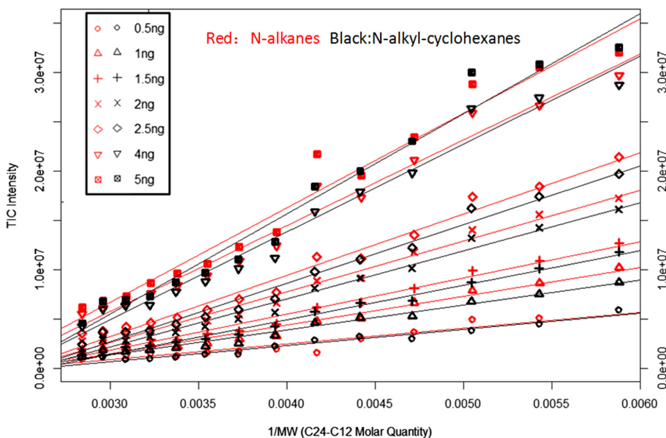
Fig. 1. TIC intensity response to the molar quantity of individual n-alkanes and n-alkyl-cyclohexanes (C 12 –C 24 ). Each line joins the TIC values for the same mass injected for compounds from C 24 (left) to C 12 (right of x-axis).
