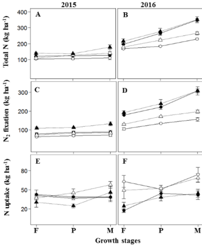
Figure 6. Total plant N content (A, B), N from N 2 -fixation in plant biomass (C, D) and N from soil N uptake in plant biomass (E, F) of two lentil genotypes “PBA Ace” (Δ, ▲ with broken lines) and “HS3010” (○, ● with continuous lines) from flowering to maturity and grown under ambient [CO 2 ] (~400 ppm, open symbols Δ ○) or elevated [CO 2 ] (~550 ppm, filled symbols ▲, ●) in the Australian Grain Free Air CO 2 Enrichment facility, Horsham, Australia during a dry (2015, left panel) and a high rainfall (2016, right panel) season. Measurements were done at flowering (F), pod filling (P) and maturity (M) stages. Means and standard errors of n=4 replicates. Statistics are reported in Table 3.
