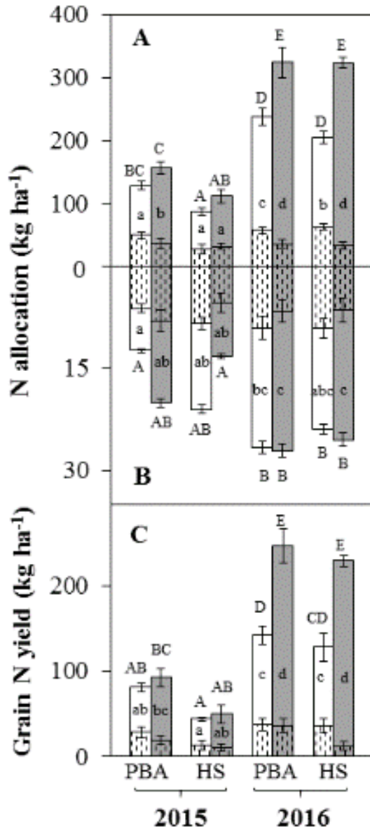
Figure 8. N allocation in above (A) and below (B) ground biomass and grain N yield (C) at maturity of two lentil genotypes “PBA Ace (PBA)” and “HS3010 (HS)” grown under ambient [CO 2 ] (~400 ppm, white bars) or elevated [CO 2 ] (~550 ppm, grey bars) in the Australian Grains Free Air CO 2 Enrichment facility, Horsham, Australia during a dry (2015, left half-panels) and a high rainfall (2016, right half-panels) season. Dotted portions refer to soil N uptake. The percentage of N derived from atmosphere (%Ndfa) is reported in Table 2. Each bar represents mean values and standard errors of n=4 replicates. Statistics are reported in Table 3. Mean values that share no common letters (upper-case for total N allocation in above, below or grain; lower-case for fixed N 2 in above, below or grain) are significantly different from each other (p < 0.05).
