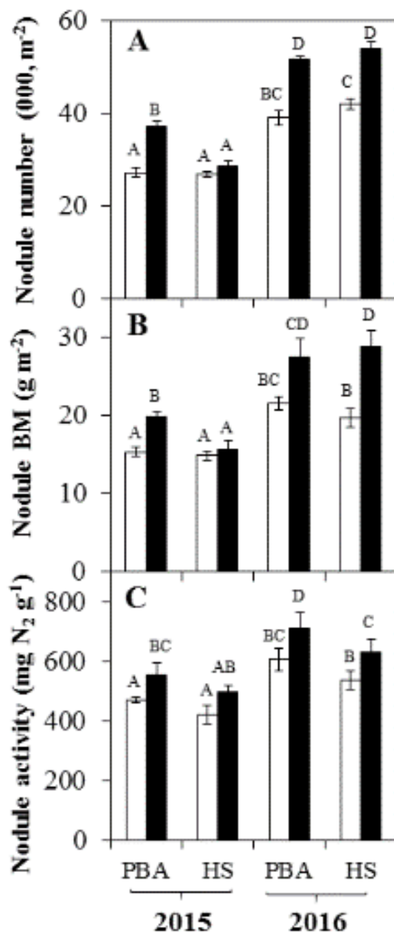
Figure 4. A. Nodule number (000, m -2 ), B. Nodule biomass (BM, dry weight basis, g m -2 ), C. Nodule activity (mg N 2 fixed g -1 nodule dry weight) of two lentil genotypes “PBA Ace (PBA)” and “HS3010 (HS)” grown under ambient [CO 2 ] (~400 ppm, white bars) or elevated [CO 2 ] (~550 ppm, black bars) in the Australian Grain Free Air CO 2 Enrichment facility, Horsham, Australia during a dry (2015) and a high rainfall (2016) season. Measurements were taken at flowering stage. Means and standard errors of n=4 replicates. Statistics are reported in Table 3. Mean values that share no common letters are significantly different from each other (p < 0.05).
