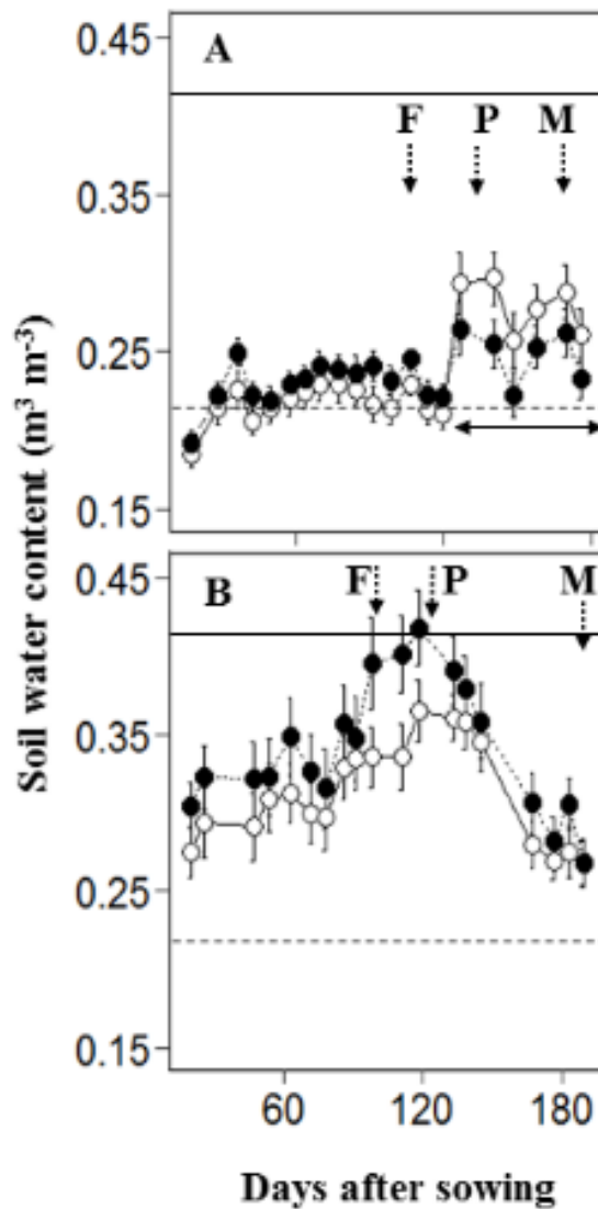
Figure 2. Volumetric soil water content ( \text{m}^3 \text{m}^{-3} ) in lentil plots in a dry (2015, A) and a high rainfall (2016, B) season under ambient [\text{CO}_2] ( \sim 400 ppm, \circ with continuous lines) or elevated [\text{CO}_2] ( \sim 550 ppm, \bullet with broken lines) in the Australian Grain Free Air \text{CO}_2 Enrichment facility, Horsham, Australia. Horizontal continuous line indicates field capacity and broken line indicates permanent wilting point. Soil water content averaged for the top 40 cm depth. Each point represents means and standard deviations of n=8 plots (two lentil genotype sub-plots in each of 4 replicate plots per [\text{CO}_2] ). Dotted arrows represent growth stages of lentil indicating flowering (F), pod filling (P) and maturity (M). Double sided arrow in the top panel (A) indicates the period receiving additional irrigation (94 mm) after flowering. Year, \text{CO}_2 and their interaction was significant at p < 0.001 ( F = 28.61 ).
