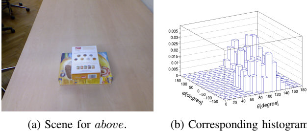
(a) Scene for above . (b) Corresponding histogram. Fig. 7: (a) Image with one object above another; and (b) corresponding histogram.
