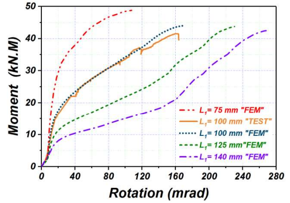
(b) M- \Phi curves for different lengths L_i of the connected angle cleats
