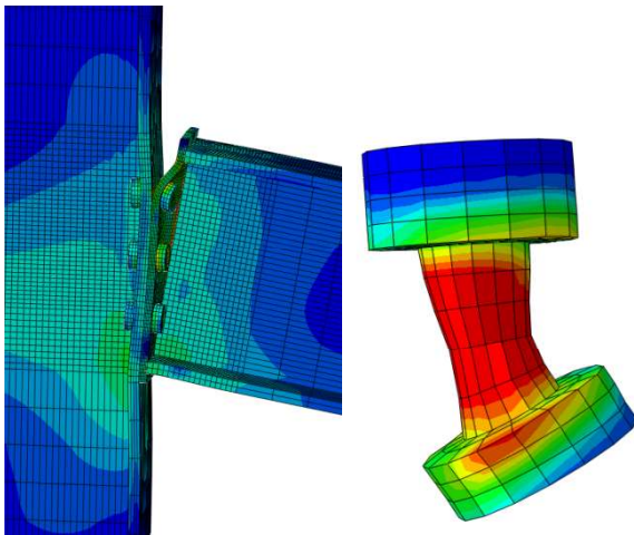
(a) Flush End Plate (FEP) connection failure mode and fractured top bolt
