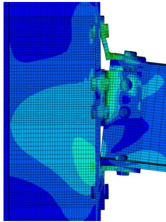
b) TSAC (g = 9 mm )
