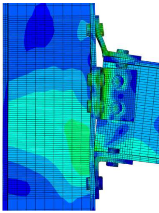
a) TSAC (g = 0 mm )
