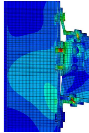
c) TSAC (g = 9 mm )
