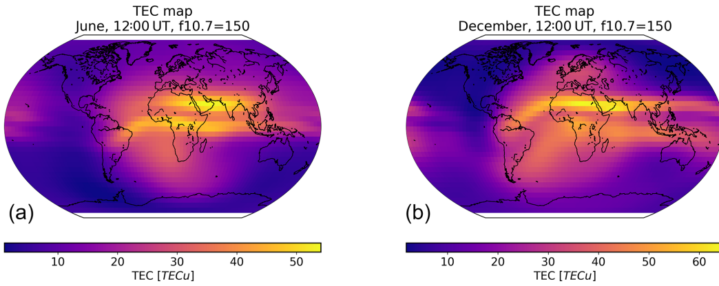
Figure 6. Vertical TEC from NeQuick for 12:00 UT, F_{10.7} = 150 : June (a) and December (b). 1\text{TECu} = 1 \times 10^{16} electrons \text{m}^{-2} .
