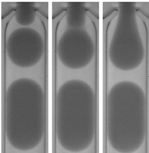
Fig. 3 – Drop coalescence at junction. Time between frames 1 ms.
