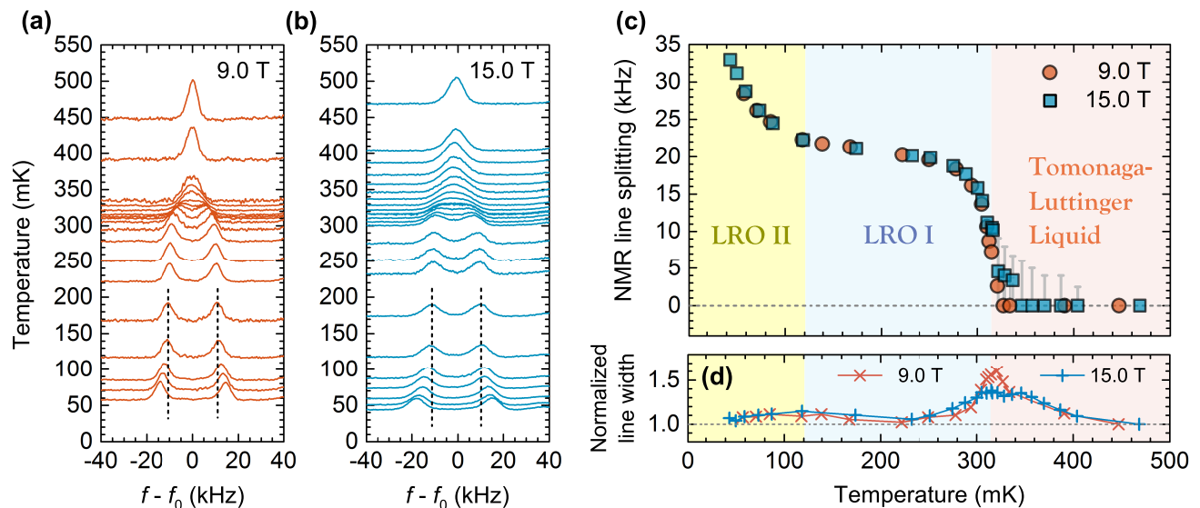
FIG. 2. (a) ^{14}\text{N} NMR spectra as a function of temperature in an applied field of 9.0 T and (b) in 15.0 T. Dashed vertical lines correspond to the first saturation of the line splittings at around 150 mK on cooling. (c) The line splitting as a function of temperature, where three different regimes are identified and presented using different background colors. (d) Normalized line width as a function of temperature.
