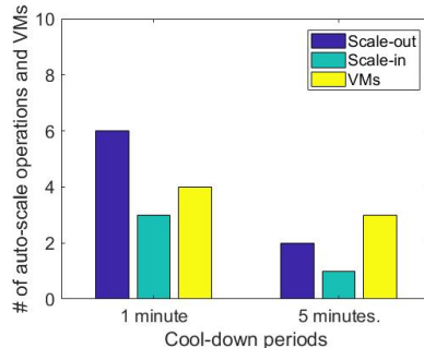
Figure 6: Auto-scale operations and VMs under the different cool-down periods.
