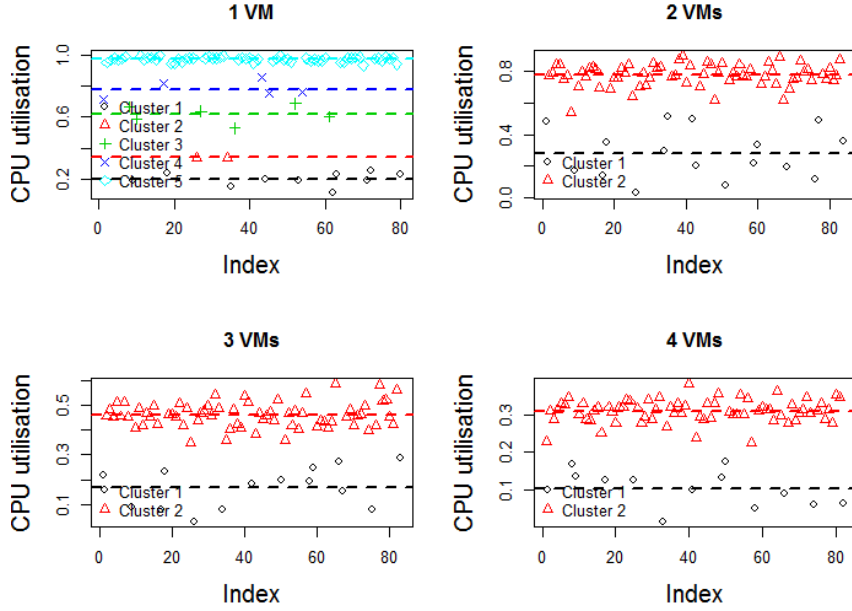
Figure 2: Optimal univariate clustering of CPU utilisation per VM number.
