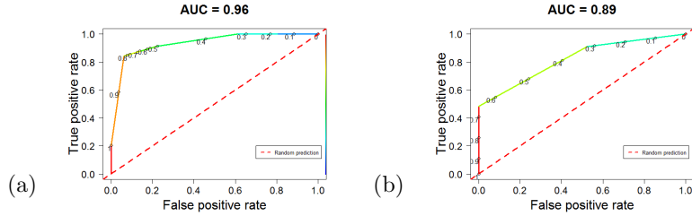
Figure 3: ROC curves under “periodic” load: (a) CPU util. viol.; (b) resp. time.
