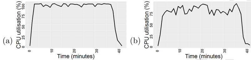
Figure 5: Sample CPU utilisation traces: (a) 1 VM; (b) 2 VMs.
