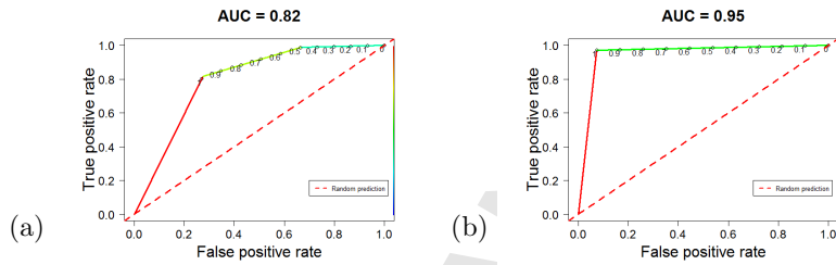
Figure 4: ROC curves under “aggressive” load: (a) CPU util. viol.; (b) resp. time.
