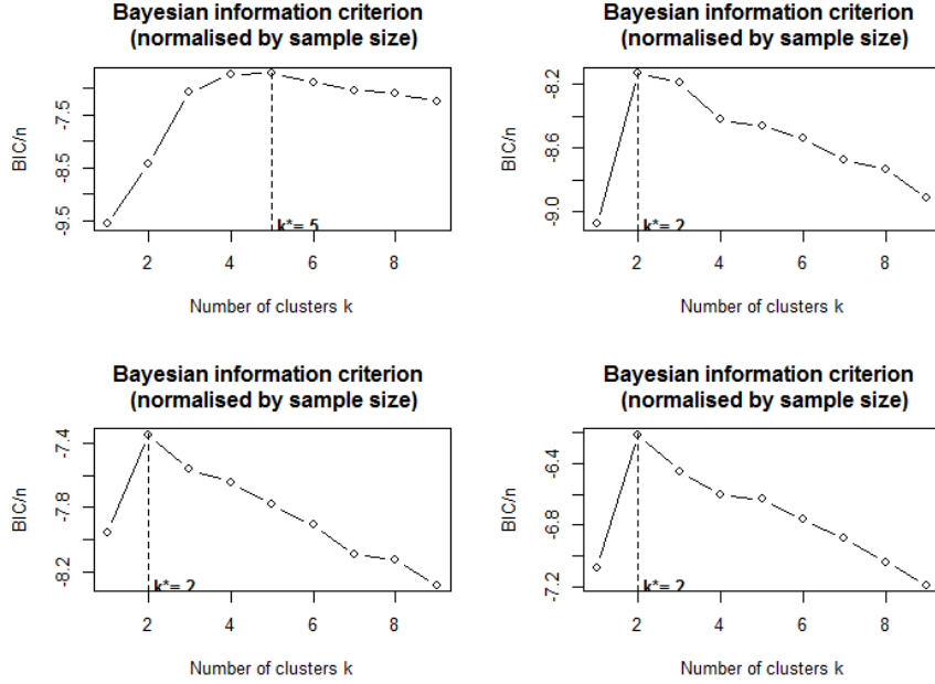
Figure 1: Determining k according to the Bayesian Information Criterion (BIC).
