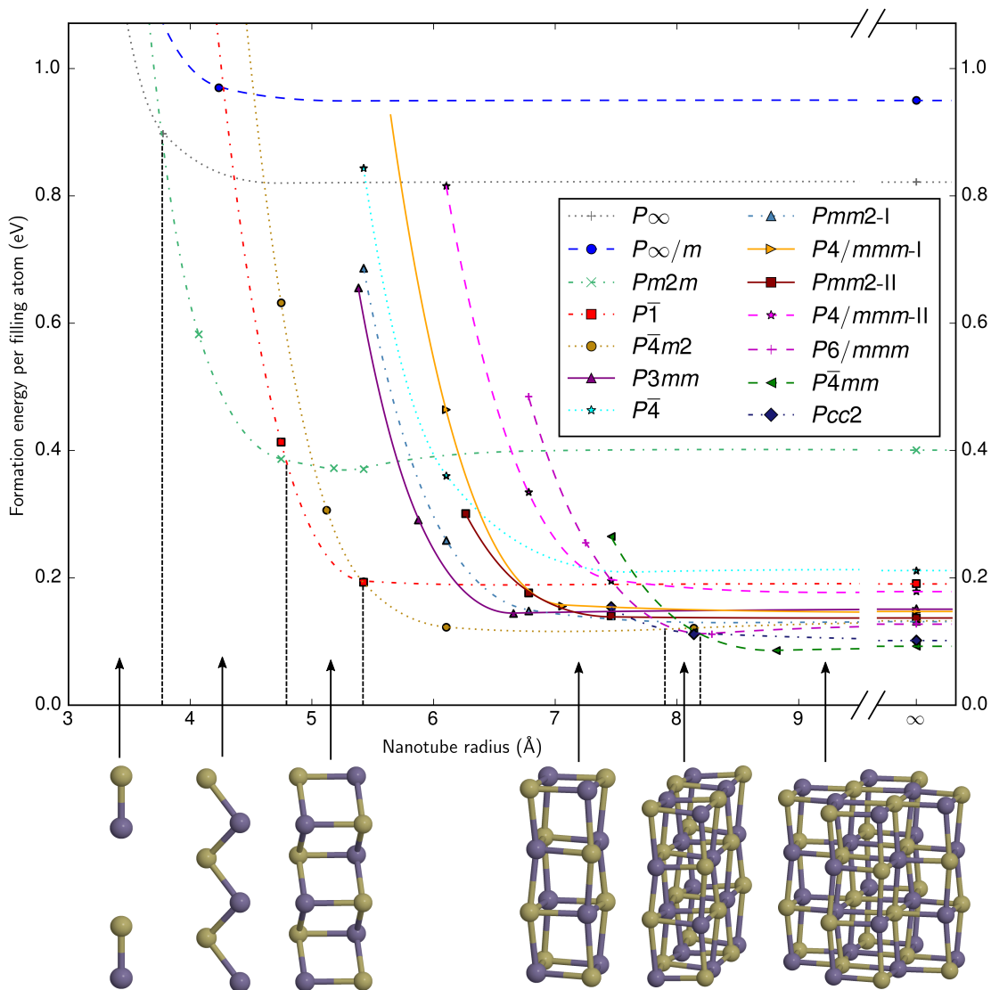
FIG. 1. Zero-temperature phase diagram for encapsulated GeTe nanowires. Where a line begins without a data point (e.g. as in the P4/mmm-I phase at 5.65 \text{ \AA} ), the structure was found to be mechanically unstable in a nanotube of that radius. In this case the energy from that calculation is not included in the fit, and the fit is then extrapolated to that point. The vertical dotted black lines indicate the positions of phase transitions at which a new nanowire phase becomes the most energetically favourable. The ground state structures are shown along the bottom, with the arrows pointing to the regions on the phase diagram at which they are the most energetically favourable structures.
