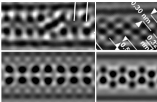
FIG. 2. A comparison between experimental TEM imagery reproduced with permission from ref. 33 (top) and simulated TEM imagery (bottom) generated from the GeTe structures predicted in this work using SimulaTEM’s ‘multislic’ package [34]. The structures shown are the P4m2 (left) and P1 (right) phases.
