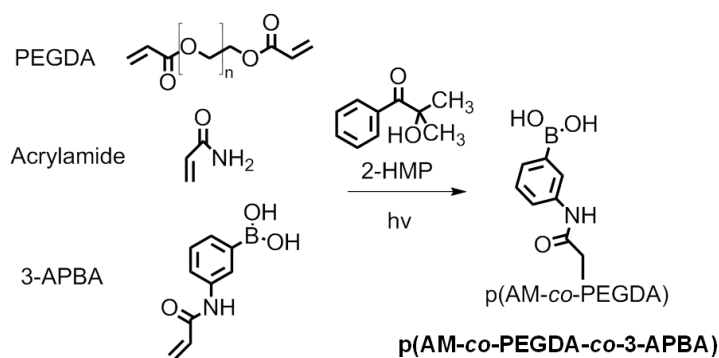
Scheme S1. Formation of p(AM-co-PEGDA-co-3-APBA) hydrogel.
