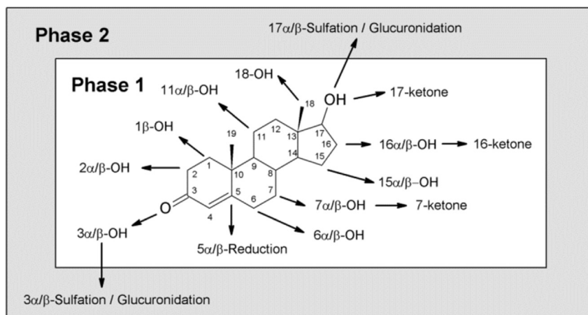
Fig. 7. Overview of hepatic phase 1 and 2 metabolism of C 19 steroids. Phase 1 metabolism comprises the 5 \alpha / \beta -reduction of the \Delta^4 double bond and the reduction of the 3-keto group to its 3 \alpha / \beta -hydroxyl as well as hydroxylations and further oxidations at various positions. Phase 2 reactions consist of the conjugation of the 3- and 17-hydroxyls. 17 \alpha -conjugates originate from Epitestosterone. The reactions shown in the figure summarize those described for T, A4 and DHEA.
