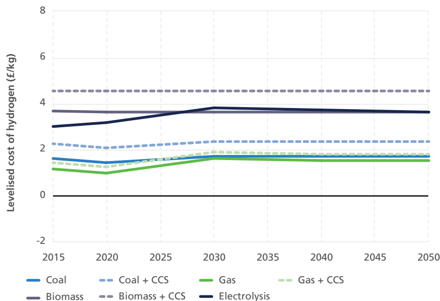
Figure S5. Levelised cost of hydrogen production forecasts for the UK from a range of sources, with a CO 2 price increasing from £50/tCO 2 in 2020 to £250/tCO 2 in 2050. No environmental levies are placed on electricity in this diagram.
