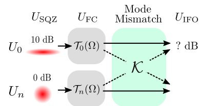
FIG. 6: The figure shows the effect of mode-mismatching the interferometer to the filter cavity and the squeezer. Initially, the vacuum noise in the spatial mode U_0 is squeezed by 10 dB, while the arbitrary higher-order mode U_n contains pure vacuum noise. The noise fields in the two spatial modes mix after being subjected to the frequency and mode dependent rotation of the squeeze angle when reflected off the filter cavity.
