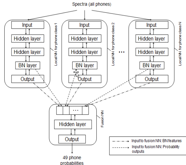
Figure 1: An architecture of the phone classification system exploiting DNN-based manifold learning of speech.
