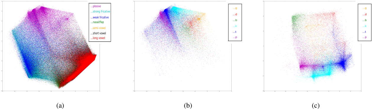
Figure 2: Visualisations of LDA-based projections of 9-dimensional bottleneck features from Q_1 ('plosive') broad phone class DNN. 1 st vs. 2 nd dimension for all data (a); 1 st vs. 2 nd dimension (b) and 3 rd vs. 4 th dimension (c) for data within plosive class only.
