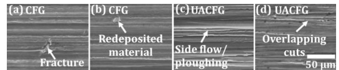
Fig. 6. SEM micrographs of \gamma -TiAl surfaces ground using SiC under (a) and (b) CFG; (c) and (d) UACFG conditions.
