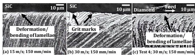
Fig. 9. Microstructures of \gamma\text{-TiAl} samples after UACFG with SiC wheel in (a) LF, (b) TF planes; and with diamond wheel in (c) LF plane.
