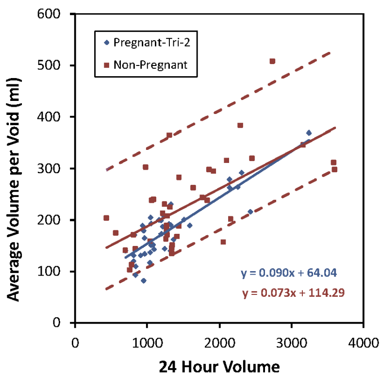
Fig 3 – Superimposed V_{avg} vs. V_{24} scatter plots with results of linear regression.
