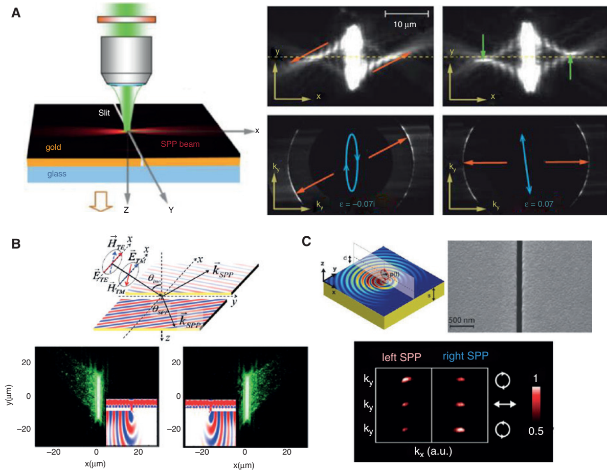
Figure 8: OSHE on a single nanoslot.
