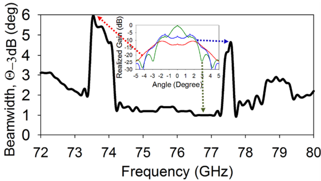
Fig. 2. Experimental beamwidth as a function of frequency. Inset: Detail of beamwidths at f = 73.5 GHz (red curve), f = 77 GHz (green curve) and f = 77.6 GHz (blue curve).
