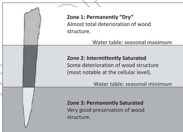
FIGURE 2 Three-zone model illustrating the link between groundwater levels and the preservation of archaeological wood. After Chapman & Cheetham (2002)
