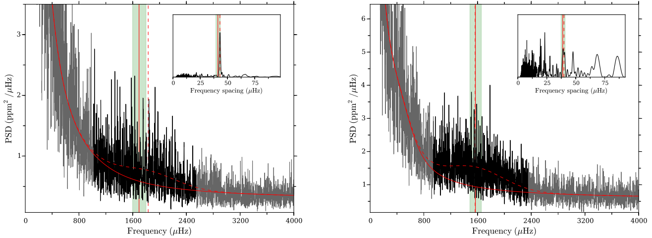
Figure 1. Power density spectra of E167 (left) and E243 (right), smoothed by a 3\ \mu\text{Hz} Epanechnikov filter. The inserts show power-of-power spectra ( \text{PS} \otimes \text{PS} ) from the region of the power spectra in black. The (full) vertical red lines indicate the spectroscopically estimated values for \nu_{\text{max}} of 1695 \pm 100\ \mu\text{Hz} (E167) and 1568 \pm 86\ \mu\text{Hz} (E243), with uncertainties given by the shaded green region; the corresponding lines in the \text{PS} \otimes \text{PS} inserts give the expected values for \Delta\nu/2 from these \nu_{\text{max}} estimates following Huber et al. (2011). Dashed vertical lines indicate the measured values for \nu_{\text{max}} and \Delta\nu (see Section 4.1). The full red lines show the obtained fits to the granulation backgrounds, with the red dashed line showing the fitted Gaussian envelope used to estimate \nu_{\text{max}} .
