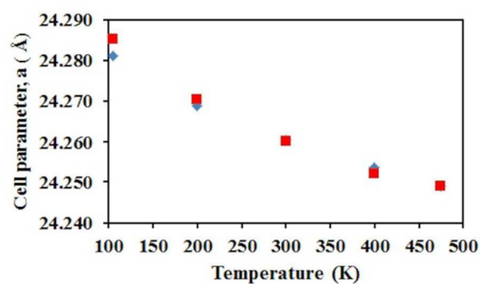
Fig. 2 The variation of unit cell parameter, a , as a function of temperature for siliceous faujasite. Red and blue data points correspond to unit cell parameters derived from the Rietveld and real-space refinements respectively. The estimated standard deviations fall in the ranges 0.0008 – 0.001 Å and 0.005 – 0.009 Å for the unit cell parameters derived from the Rietveld and real-space refinements respectively and are provided in the ESI.
