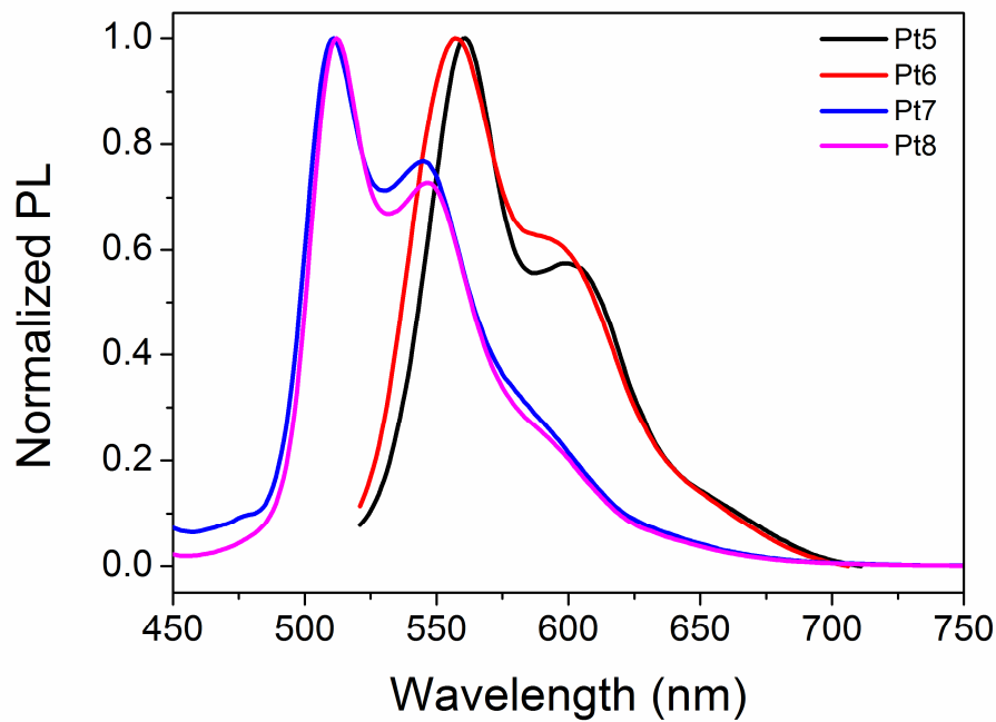
Figure 4 PL spectra (excitation at 420 nm) of platinum complexes in CH 2 Cl 2 at room temperature.
