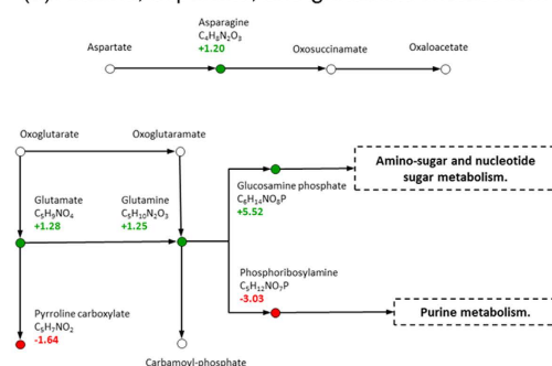
(a) Alanine, aspartate, and glutamate metabolism
