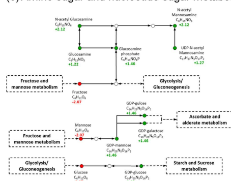
(c) Amino sugar and nucleotide sugar metabolism
