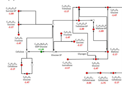
(b) Starch and sucrose metabolism
