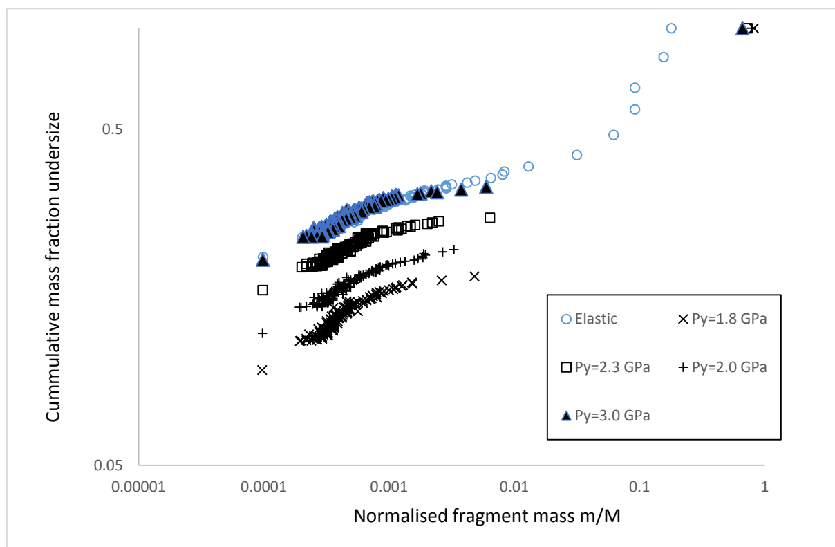
Fig. 10 Fragment size distributions for V = 2 m/s
