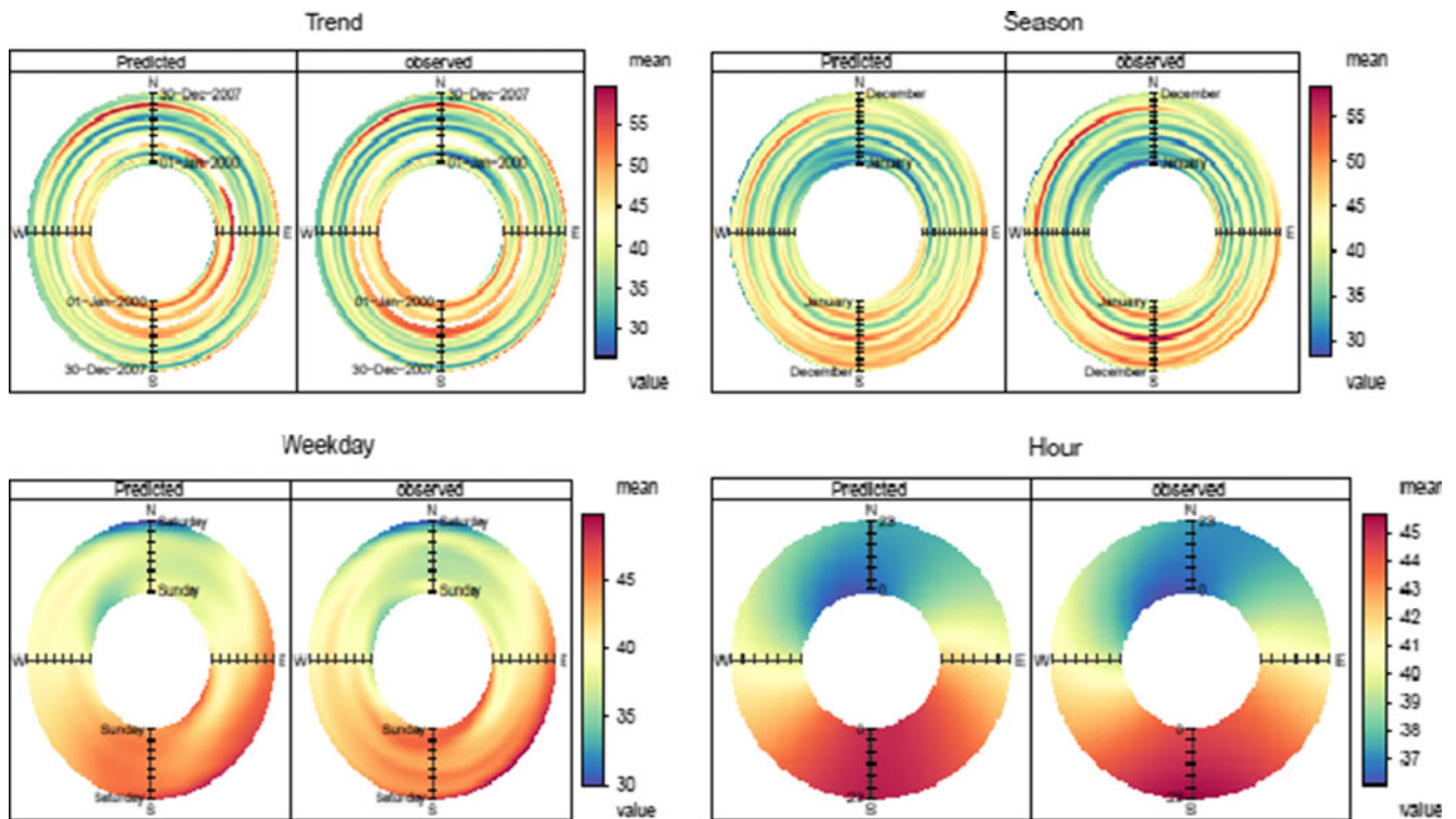
Fig. 13 Comparison between the observed and ANNElasticNET-predicted PM 10 concentrations
