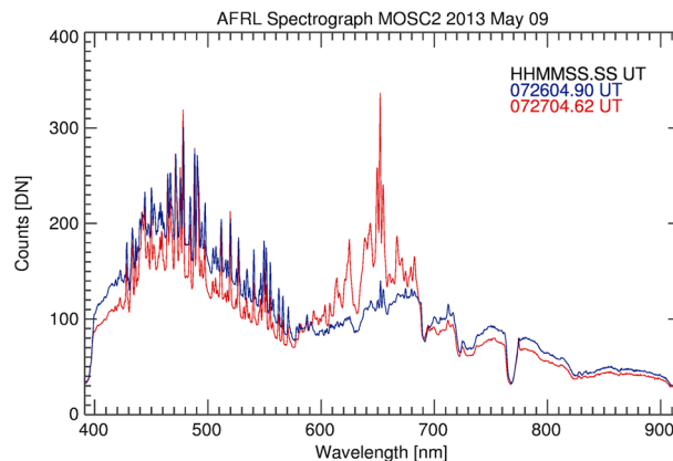
Figure 7. Spectra from MOSC-2 immediately after (blue) and 1 min after (red) release produced by averaging the central 200 pixels in the spatial dimension of the acquired 1340 \times 400 images.
