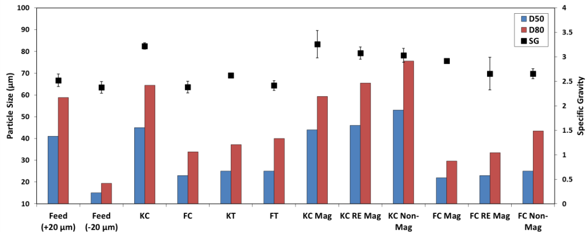
Figure 4 – Particle sizes ( d_{50} and d_{80} values determined by QEMSCAN) and specific gravities of different products of centrifugal gravity concentration and drum magnetic separation. Error bars represent 95 % confidence intervals
