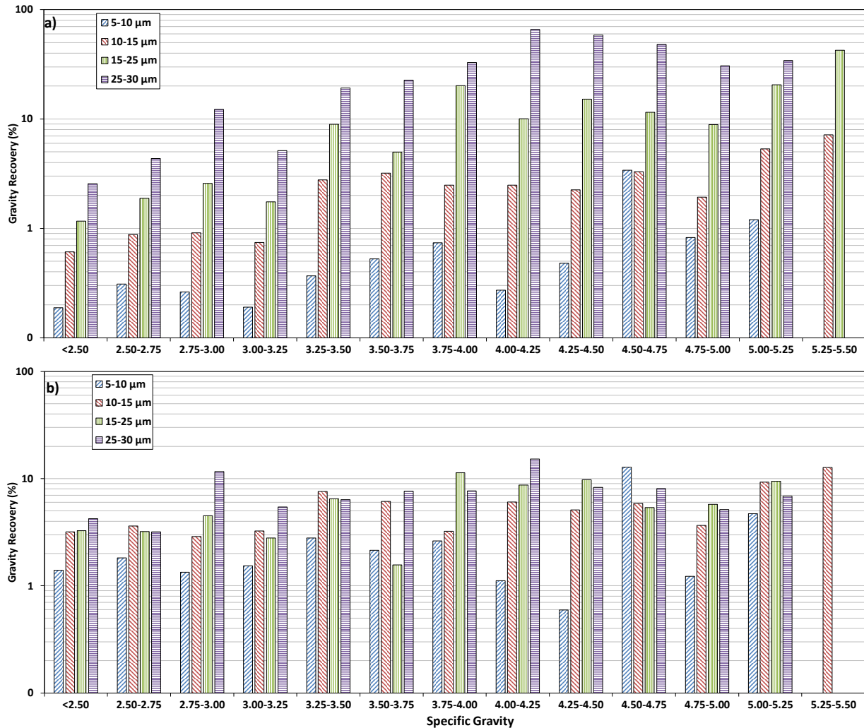
Figure 7 – Gravity recovery for small (<30 μm) particles across particle specific gravity size classes for a) Knelson gravity concentrate and b) Falcon gravity concentrate
