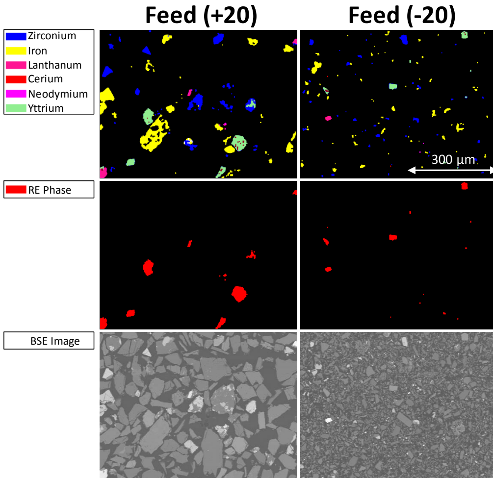
Figure 12 – SEM images of the feed (+20 μm and -20 μm) to gravity and magnetic separation including elemental (Zr, Fe, La, Ce, Nd, Y) phase identification, REM phase identification and backscattered electron (BSE) images
