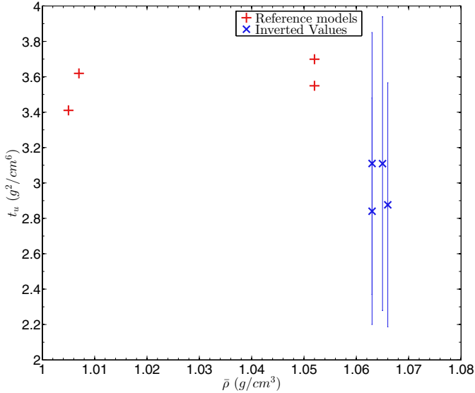
Fig. 6. t_u inversion results for 16CygB. The red + are the reference models and the blue × the inverted results. The lower + are associated with the upper × and refer to models including solar-calibrated diffusion.
