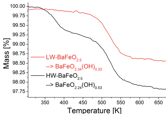
Fig. 3 TG experiments performed on the hydrated modifications of BaFeO 2.5 under flowing argon.
