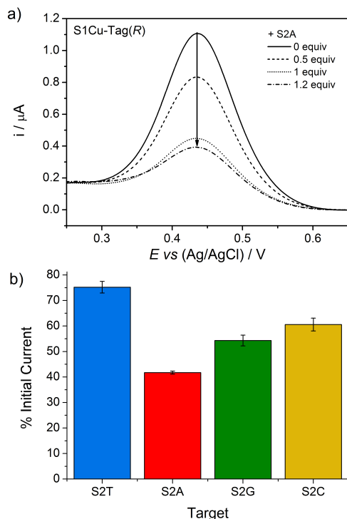
Figure 4. a) Square wave voltammetry current changes for Cu-Tag(R) bound to increasing molar equivalents of S2A ; b) Percentage current change at i_{\max} for duplexes with each of the four canonical bases opposite tag. Error bars represent the S.E.M. [DNA] = 50 \mu\text{M} in 10 mM tris-HCl buffer (pH 7), 100 mM NaCl, 293 K.
