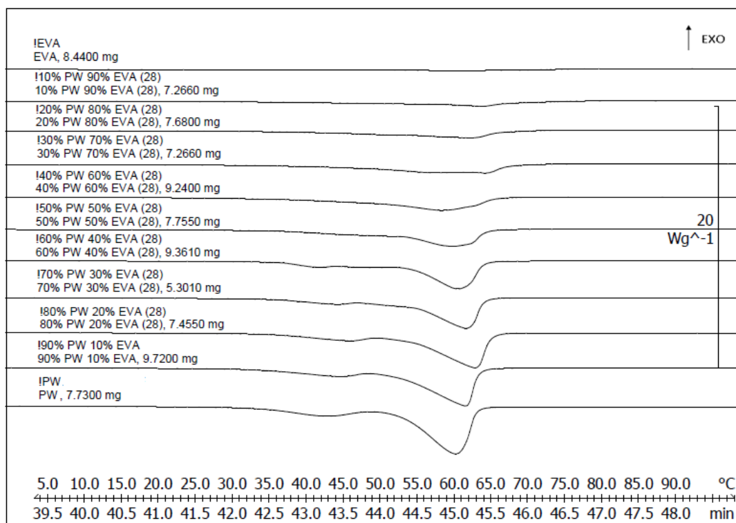
Figure 5: DSC analysis of paraffin wax and ethylene vinyl acetate blend (data from heating cycle 2, -20\text{ }^{\circ}\text{C} to 600\text{ }^{\circ}\text{C} at a rate of 10\text{ }^{\circ}\text{C min}^{-1} ).
