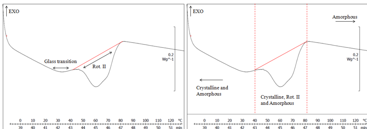
Figure 4: DSC heating trace of EVA (heating rate of 10^\circ\text{C}\cdot\text{min}^{-1} ) describing transitions (left) and state of material (right) with increasing temperature.
