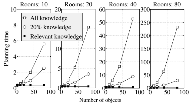
Figure 3: Planning time as a function of the number of rooms and the number of objects in the domain—PA scales to larger number of rooms and objects.
