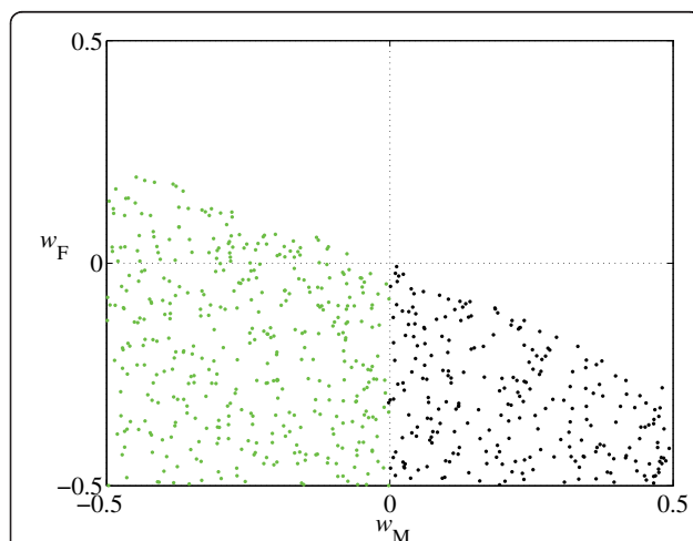
Figure 6 Protected polymorphism and fitness. The mutation pair a \rightarrow A/f \rightarrow f in Region II (Figure 5(a)) either leads to recruitment of f (black points) when selection favors higher expression in males ( w_M > 0 ) or protected polymorphism (green points) when selection favors lower expression in males ( w_M < 0 ).
