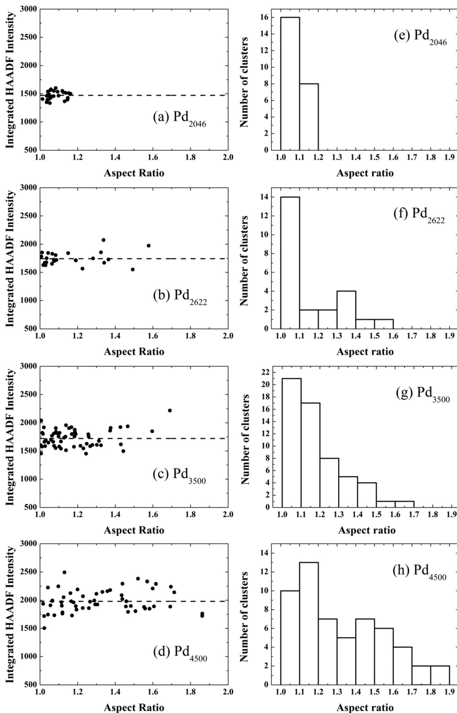
Fig. 2 Integrated HAADF image intensity from individual (a) Pd 2046 , (b) Pd 2622 , (c) Pd 3500 , and (d) Pd 4500 clusters as a function of their aspect ratio. Data points represent individual clusters of the respective size. The dashed lines show the average integrated HAADF intensity values for the corresponding cluster size. Histograms of cluster aspect ratios are presented in (e)–(h) for Pd 2046 , Pd 2622 , Pd 3500 , and Pd 4500 clusters, respectively.
