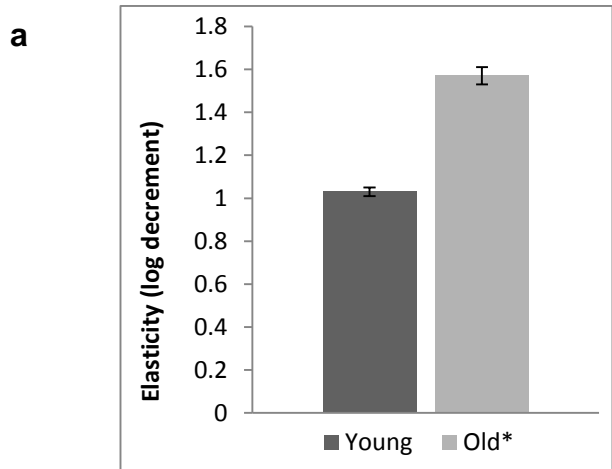
Figure 3. Differences in rectus femoris muscle parameters between healthy young and older adults measured using the MyotonPRO device. a) elasticity; b) tone; c) stiffness. *significant difference between groups p < 0.001
