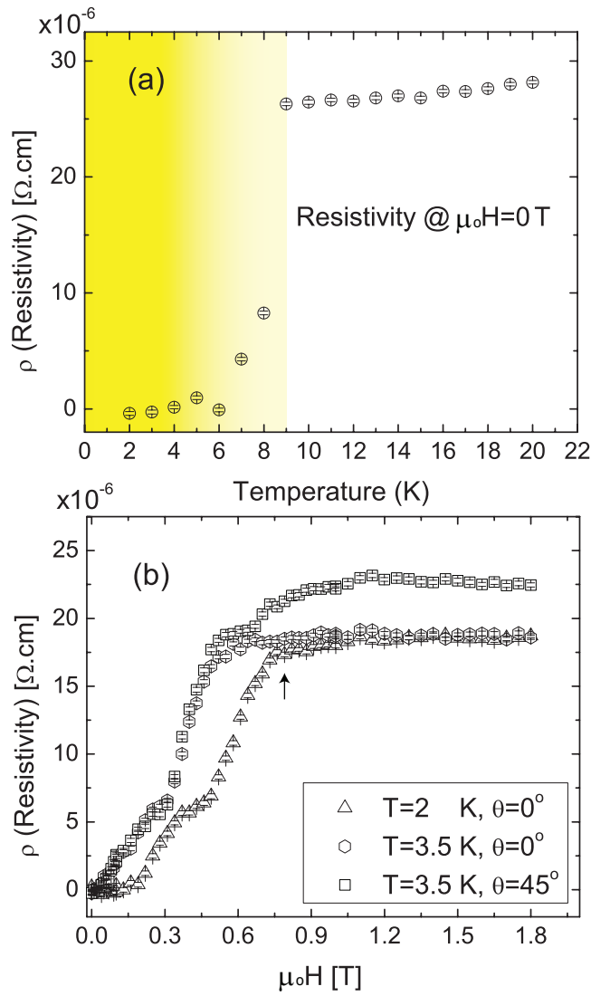
Fig. 1 Resistivity \rho measurements as functions of temperature T and of magnetic field H . (a) shows \rho(T) at zero field; (b) shows \rho(H) at T = 2 K and T = 3.5 K, with fields \mathbf{H} applied parallel to \mathbf{c} and also at 45^\circ to \mathbf{c} in the (110) plane. The arrow shows the point for H_{c2}(T=2\text{K}) of the previous study [10]. In (a) the yellow background shading highlights the superconducting region.
