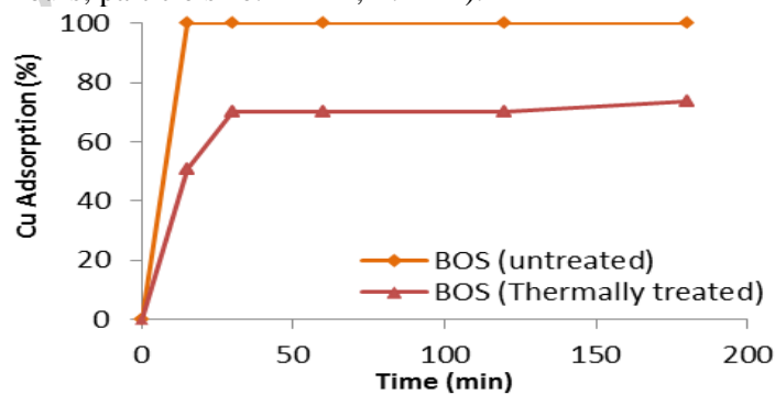
Fig. 9: Effect of thermally treated BOS sludge on its capacity to remove Cu ions from Wheal Jane mine AMD.
