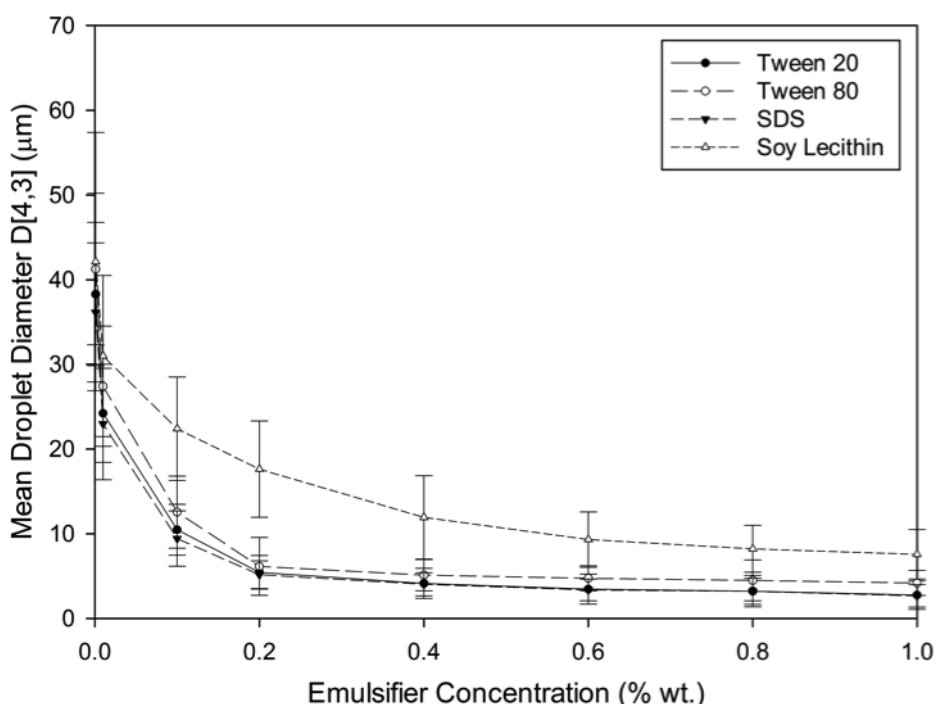
Figure 3. The effects of the concentration of different emulsifiers on the droplet size produced at 10 kPa and 1000 rpm with a rotating membrane emulsification system.
