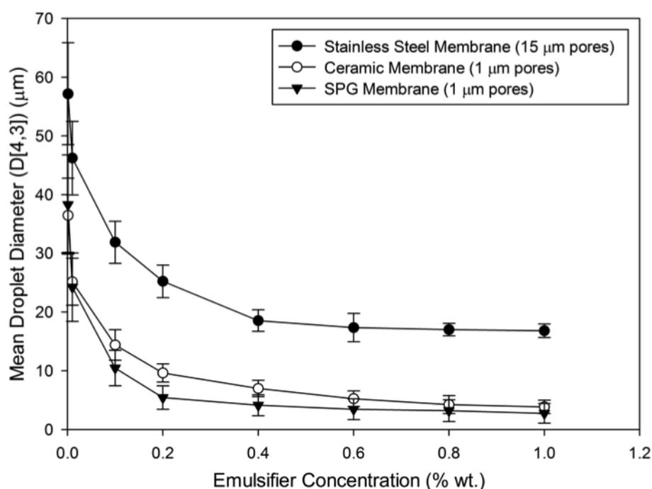
Figure 4. The effects of different concentrations of Tween20 on the droplet sizes produced from the three different rotating membranes at 10 kPa and 1000 rpm.
