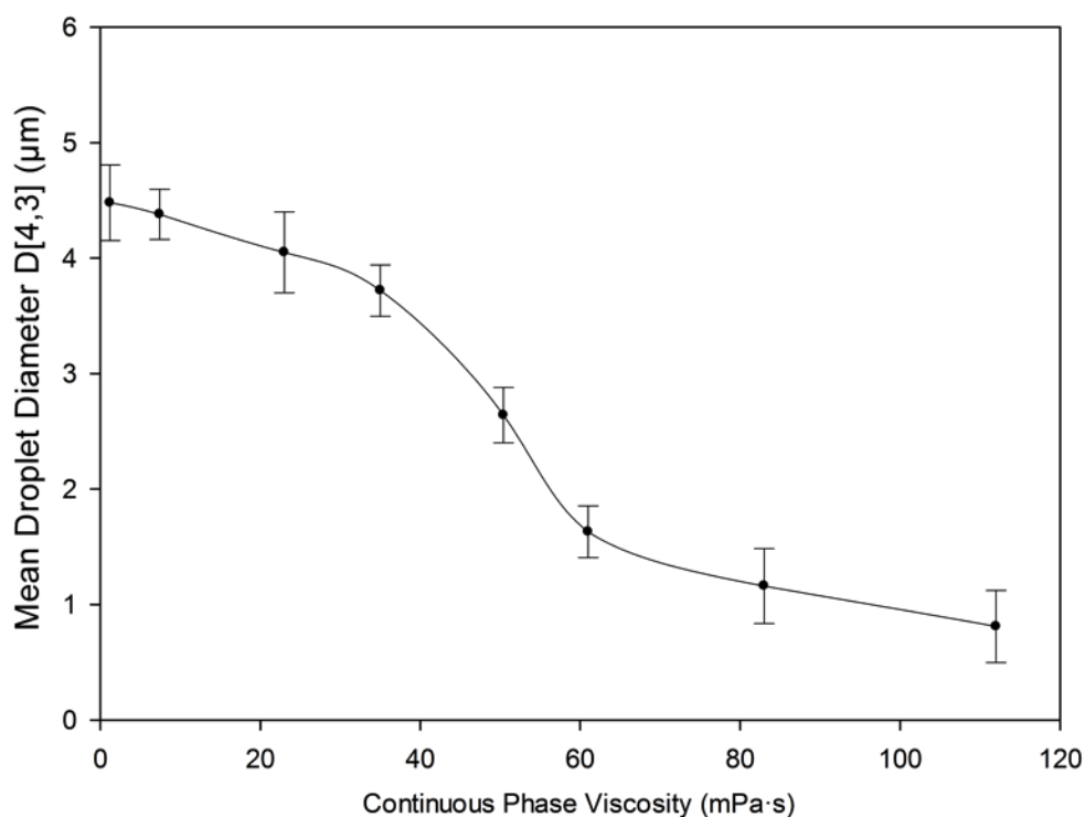
Figure 9. The effects of continuous phase viscosity changes on droplet size. The droplets were produced using a 1 \mu\text{m} SPG membrane at 10 kPa trans-membrane pressure and 1000 rpm, at 1% dispersed phase volume and 1% tween 20 emulsifier.
