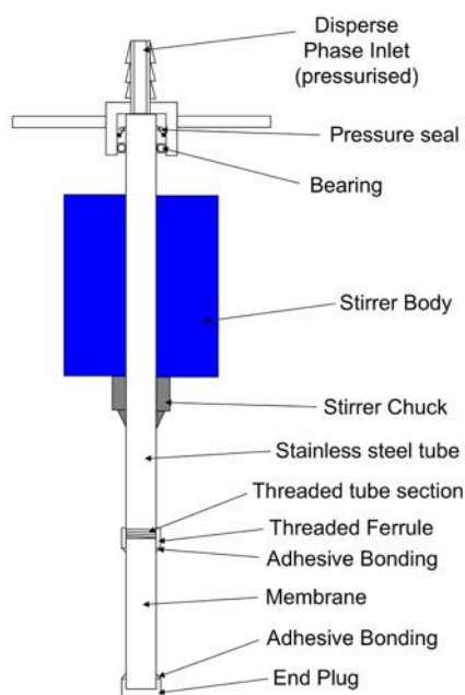
Figure 1. The rotating membrane emulsification system employed a rotating fluid coupling to allow pressurised fluid to flow into the shaft and on into the rotating tubular membrane. The continuous phase was housed in a suitable vessel in which the membrane was submerged.
