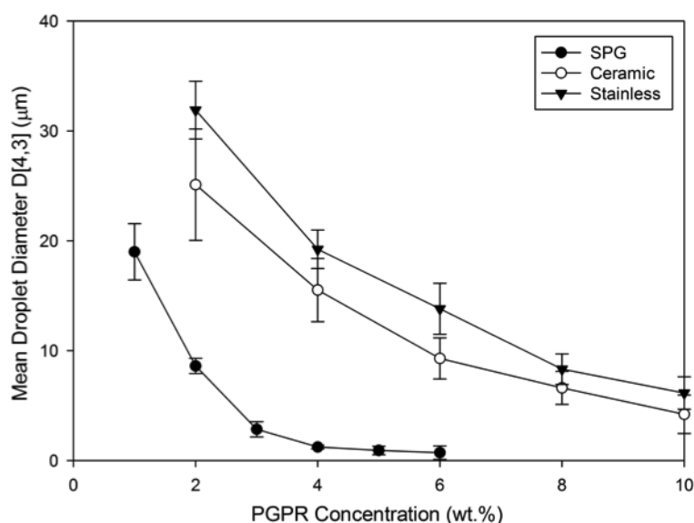
Figure 10. The effect of emulsifier concentration on the size of water in oil droplets produced using rotating membrane emulsification. The emulsions were made to 1% phase volume at 10 kPa and 1000 rpm.
