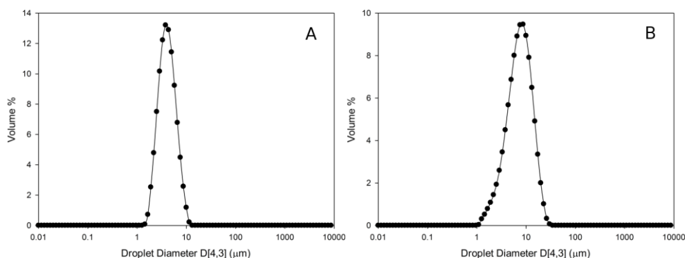
Figure 8a and 8b. A shows the droplet size distribution at 10 kPa 1000 rpm with 1% oil phase volume and 1% Tween 20 as the emulsifier with a 1 \mu m ceramic membrane, and b shows the same emulsion produced at 200 kPa. The relative span of a is 1.13 and of b is 1.54.
