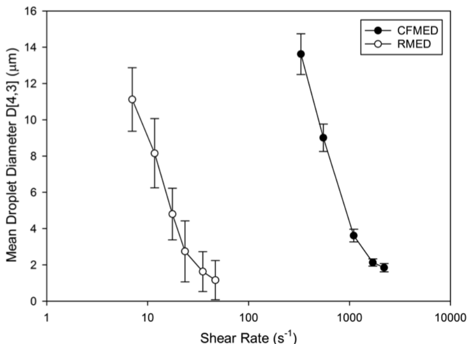
Figure 5. The effects of shear rate on the droplet sizes produced via cross-flow membrane emulsification device (CFMED) and rotating membrane emulsification device (RMED). The membranes are similar 1 \mu m SPG, with 1% tween20 and 1% oil phase volume.
