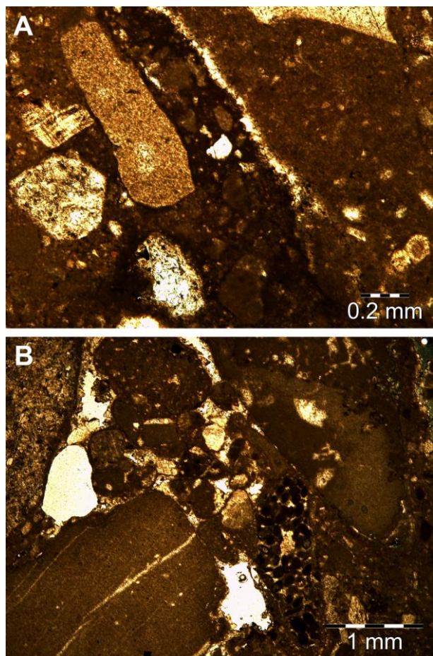
Fig. 4. Thin sections of consolidated tills from Rujno paleoglacier. A) JV-JM till showing fabric with parallel orientation of elongated clasts. B) VR-RK till showing lack of any preferential orientation of clasts.
