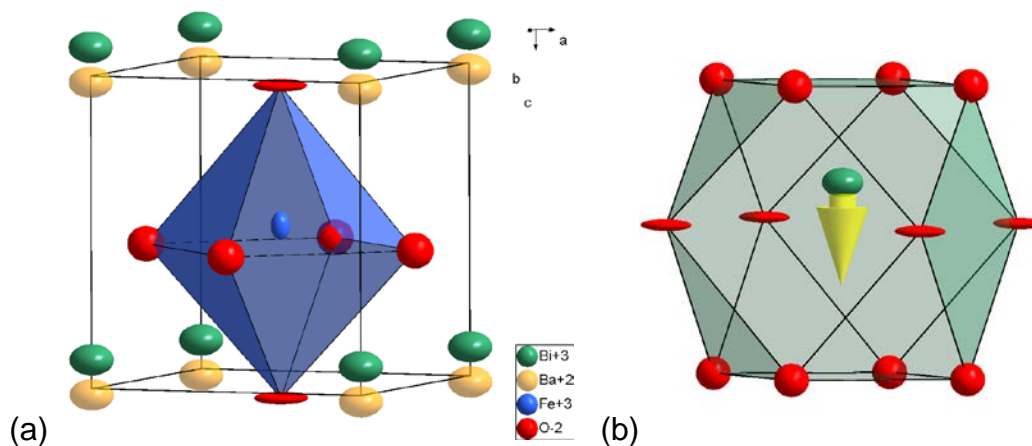
Figure 6. Refined crystal structure together with thermal ellipsoids for the different ions of \text{Bi}_{0.8}\text{Ba}_{0.2}\text{FeO}_{2.8}\text{F}_{0.2} (a). The location of Bi ion (green) in its anion (red) coordination polyhedron together with the mutual position (as found for \text{PbTiO}_3 87 ) of the lone pair indicated by an yellow arrow (b). For a detailed analysis of the lone pair position, DFT based calculations would be required.
