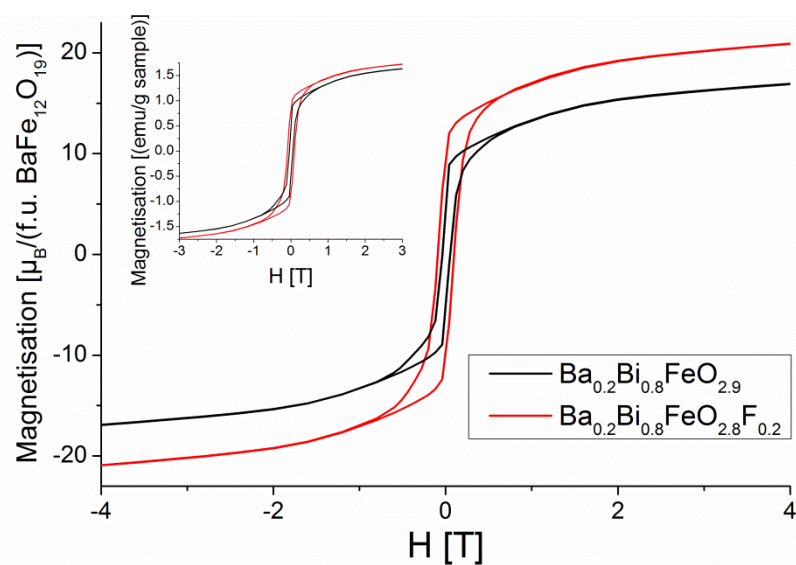
Figure 9. Field dependent measurements of the magnetisation of \text{Bi}_{0.8}\text{Ba}_{0.2}\text{FeO}_{2.9} and \text{Bi}_{0.8}\text{Ba}_{0.2}\text{FeO}_{2.8}\text{F}_{0.2} (inlay), measured magnetisation correlated with the amount of \text{BaFe}_{12}\text{O}_{19} determined by quantitative phase analysis of the NPD data.
