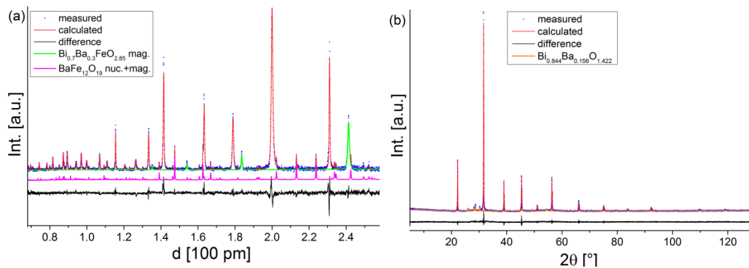
Figure 1. Rietveld analysis of the nuclear and magnetic structure of \text{Bi}_{0.8}\text{Ba}_{0.2}\text{FeO}_{2.9} . HRPD bank 1 (a) and XRD (b) data are shown. HRPD bank2 and bank3 data are provided as Figure S1a and Figure S1b in the Supplementary Material.
