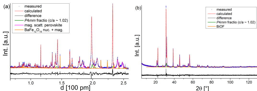
Figure 5. Rietveld analysis of the nuclear and magnetic structure of \text{Bi}_{0.7}\text{Ba}_{0.3}\text{FeO}_{2.7}\text{F}_{0.3} (unknown reflection at d = 3.415\text{-}3.420 is marked with *). HRPD bank 1 (a) and XRD (b) data are shown. HRPD bank2 and bank3 data are provided as Figure S4a and Figure S4b in the Supplementary Material.
