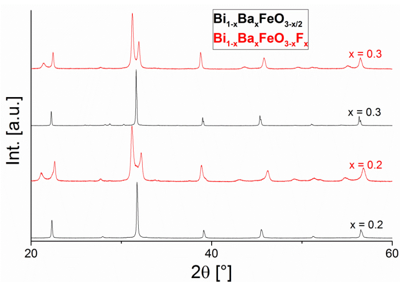
Figure 3. XRD patterns of the oxide and oxyfluoride compounds \text{Bi}_{1-x}\text{Ba}_x\text{FeO}_{3-x/2} and \text{Bi}_{1-x}\text{Ba}_x\text{FeO}_{3-x}\text{F}_x . Apart from the perovskite compound, a small impurity of \text{BiOF} was detected for both compositions, which is likely to be formed from the impurity of tetragonal \text{Bi}_2\text{O}_3 (or \text{Bi}_{0.844}\text{Ba}_{0.156}\text{O}_{1.422} ) since the respective amounts compare very well. In the neutron diffraction pattern, the small amount of the ferrimagnetic impurity \text{BaFe}_{12}\text{O}_{19} also
