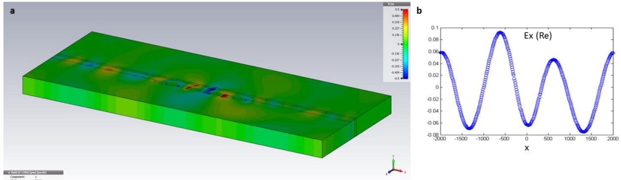
Figure 2. a – 3-dimensional colourmap of the x-component of the E-field at 280 THz for the metalens simulation with a grating sample. The x-component of the E-field is shown here as it is the main component of the overall E-field, due to the incident light being y-polarised which the metalens converts into predominantly x-polarised light; b – Plot of the real component of the x-component of the electric field data along a line in the x-direction at the end of the simulation volume ( y=0, z=2000\text{nm} ), processed in MATLAB. This corresponds qualitatively with the CST simulation.
