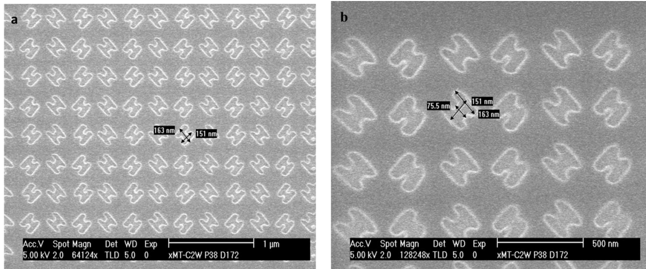
Figure 3. SEM images of: a –the unit cell array of ‘H’ shapes; b – zoomed in SEM image of the unit cell array of ‘H’ shapes.
