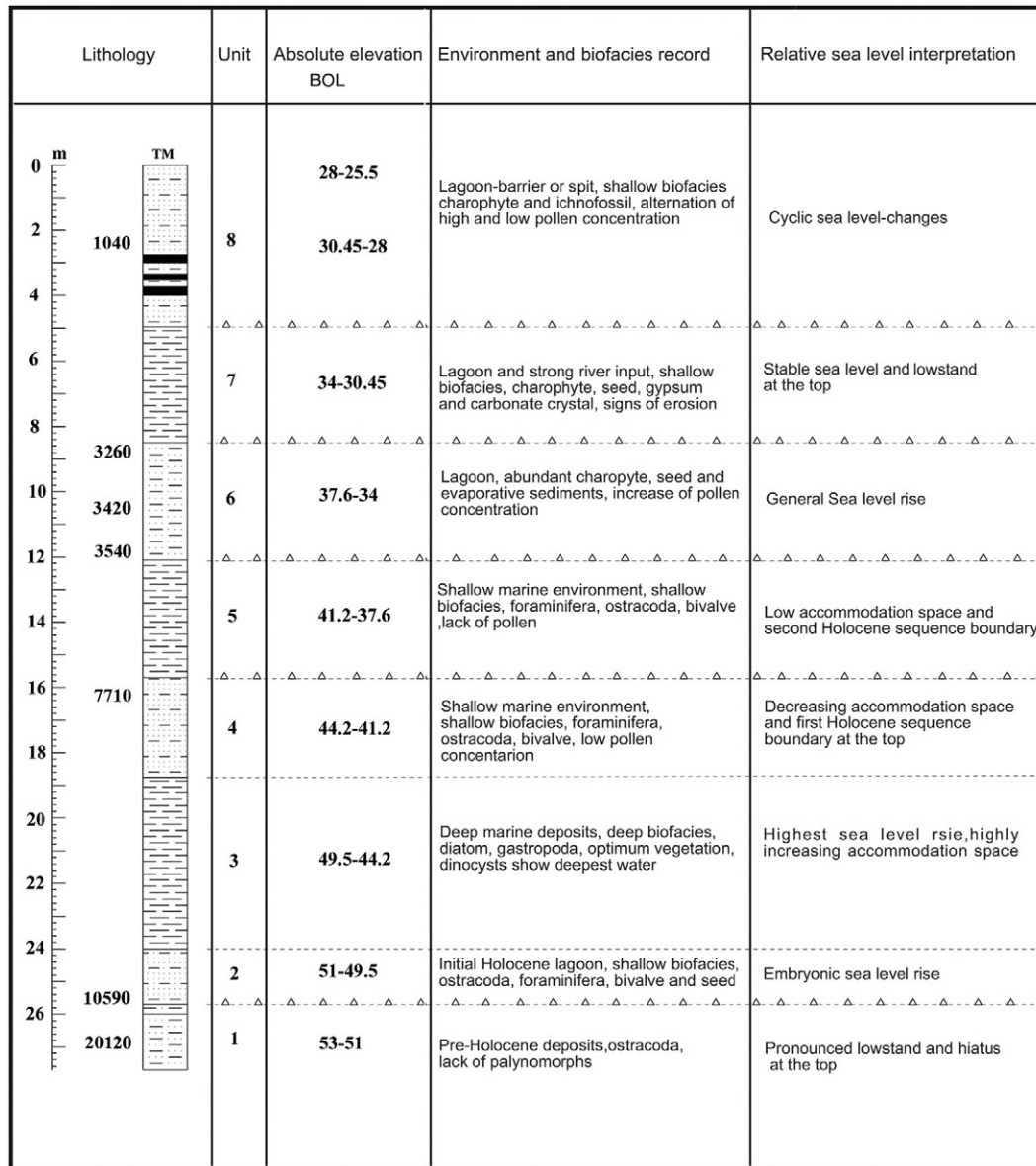
Fig. 9. Sea-level interpretation of the Late Pleistocene to Holocene time associated with biofacies and sedimentology data from core TM. The lines with triangles indicate the sequence boundaries.
