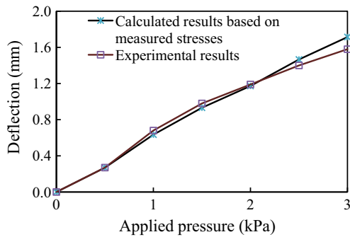
Fig. 8. Maximum deflections of the upper glass panel with increasing uniform pressure.
