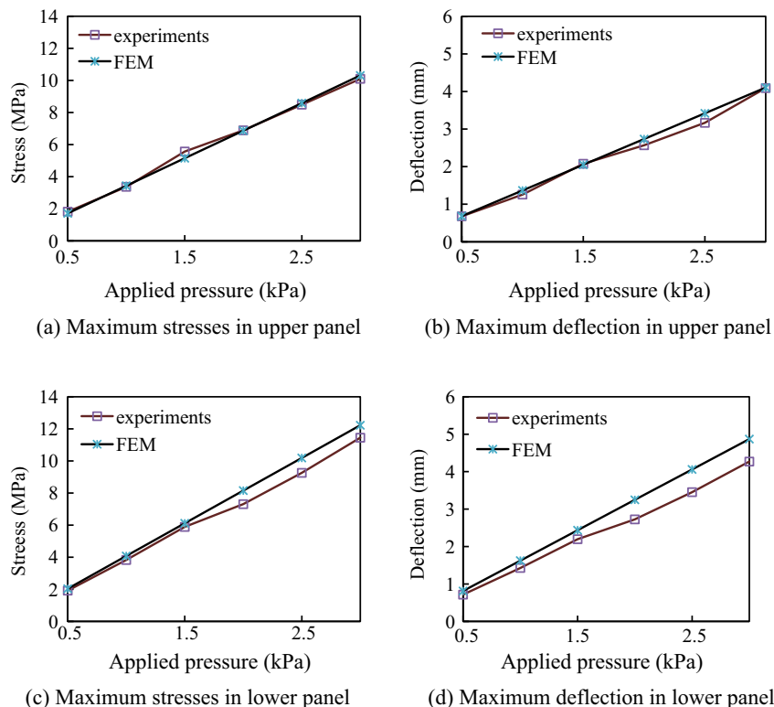
Fig. 12. Comparison of maximum stresses and deflections for Design II.
