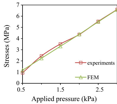
(a) Maximum stresses in upper panel
