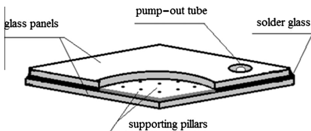
Fig. 1. Schematic diagram of vacuum glazing [9].
