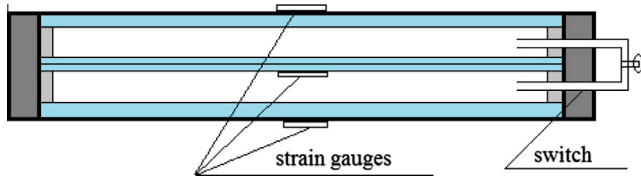
Fig. 4. Schematic diagram of the specimen with switchable pressure equalisation valve.
