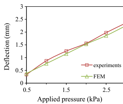
(f) Maximum deflections in lower panel
