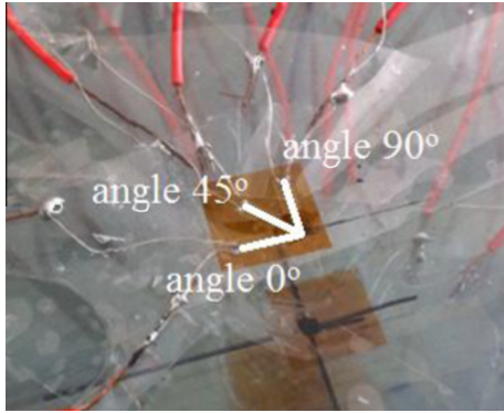
Fig. 3. Strain gauge rosette glued on glass surface.
