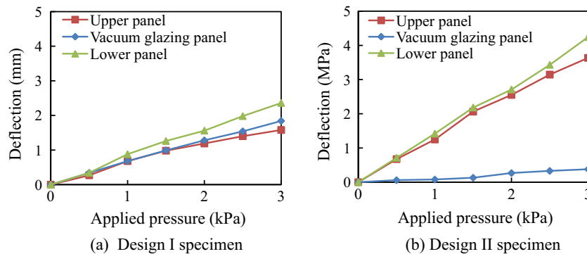
Fig. 9. Deflections of each glass panel in two glazing designs.
