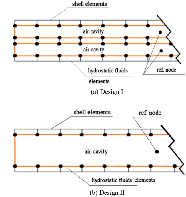
Fig. 10. Schematic diagrams of numerical models for both designs.
