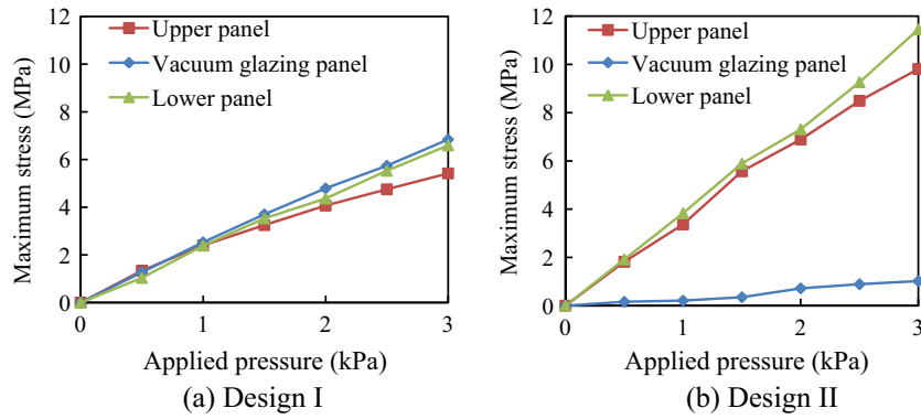
Fig. 7. Stresses measured for each glass panel.
