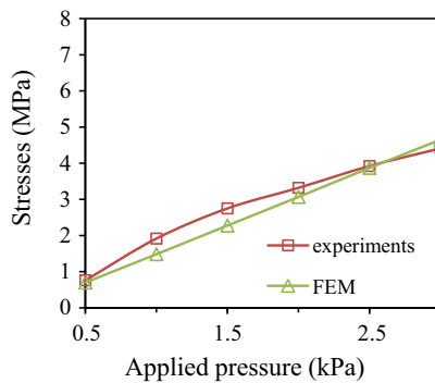
(e) Maximum stresses in lower panel
