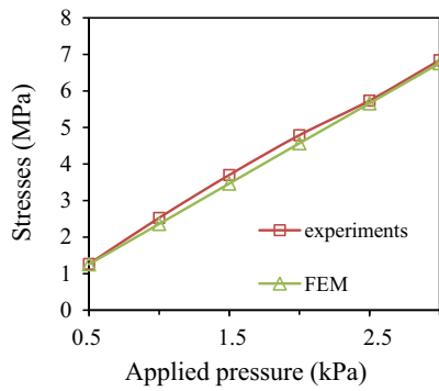
(c) Maximum stresses in VGU panel
