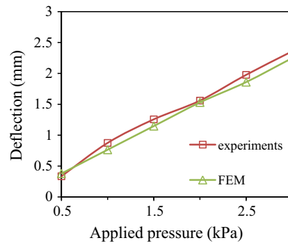
(b) Maximum deflections in upper panel
