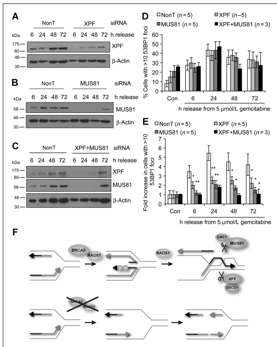
Figure 6. Gemcitabine-induced DSBs depend on MUS81 and XPF. A , protein levels of XPF and \beta -actin (loading control) after transfection with nonT or XPF siRNAs for 72 hours, treated with 5 \mu M/L gemcitabine for 2 hours and release for the times indicated. B , protein levels of MUS81 after transfection with nonT or MUS81 siRNAs as in A . C , protein levels of XPF, MUS81, and \beta -actin (loading control) after transfection with nonT or MUS81 and XPF siRNAs as in A . D , percentage of U2OS cells \pm XPF and MUS81 displaying more than 10 53BP1 foci after release from gemcitabine. E , quantification of increase in cells displaying more than 10 53BP1 foci as in D (asterisks compared with nonT siRNA). F , suggested model for HR-dependent replication fork slowing and DSB formation. Forks affected by gemcitabine treatment are recognized by BRCA2 and RAD51 and remodeled into joint molecule HR intermediates such as D-loops. These intermediates are preferentially cleaved by MUS81 and XPF. Error bars, SEM; *, P < 0.05 ; **, P < 0.01 , Student t test.
