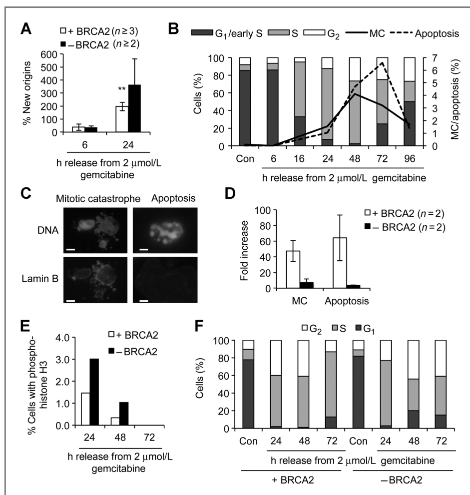
Figure 2. BRCA2-deficient and -proficient cells display aberrant cell-cycle progression after release from gemcitabine. A, new origin firing in VC8 and VC8-B2 cells after release from gemcitabine. DNA fiber labeling was performed as in Fig. 1D and IdU-only labeled tracks (new origins) were normalized to all CldU-containing tracks. B, FACS analysis of cell-cycle progression and time course of mitotic catastrophe (MC) and apoptosis in VC8-B2 cells after release from gemcitabine. C, representative images of DAPI- and Lamin B1-stained VC8-B2 cells with mitotic catastrophe or apoptotic phenotypes after 48-hour release from gemcitabine. Bars, 10 \mu m. D, increase in MC and apoptosis in VC8 and VC8-B2 cells after release from 5 \mu mol/L gemcitabine. E, percentages of VC8-B2 and VC8 cells positive for phospho-histone H3 staining following release from gemcitabine in the presence of 1.5 \mu mol/L nocodazole. F, cell-cycle progression in VC8 and VC8-B2 cells after release from 5 \mu mol/L gemcitabine for 24 to 72 hours. Error bars, SEM; **, P < 0.01 , Student t test.
