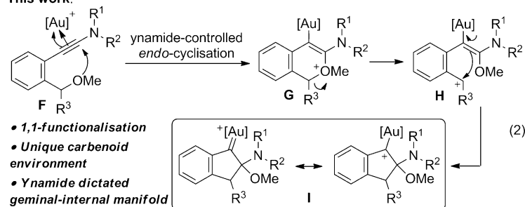
Scheme 2. Gold-catalysed carboalkoxylation: proposed ynamide-dictated carboalkoxylation mode.
